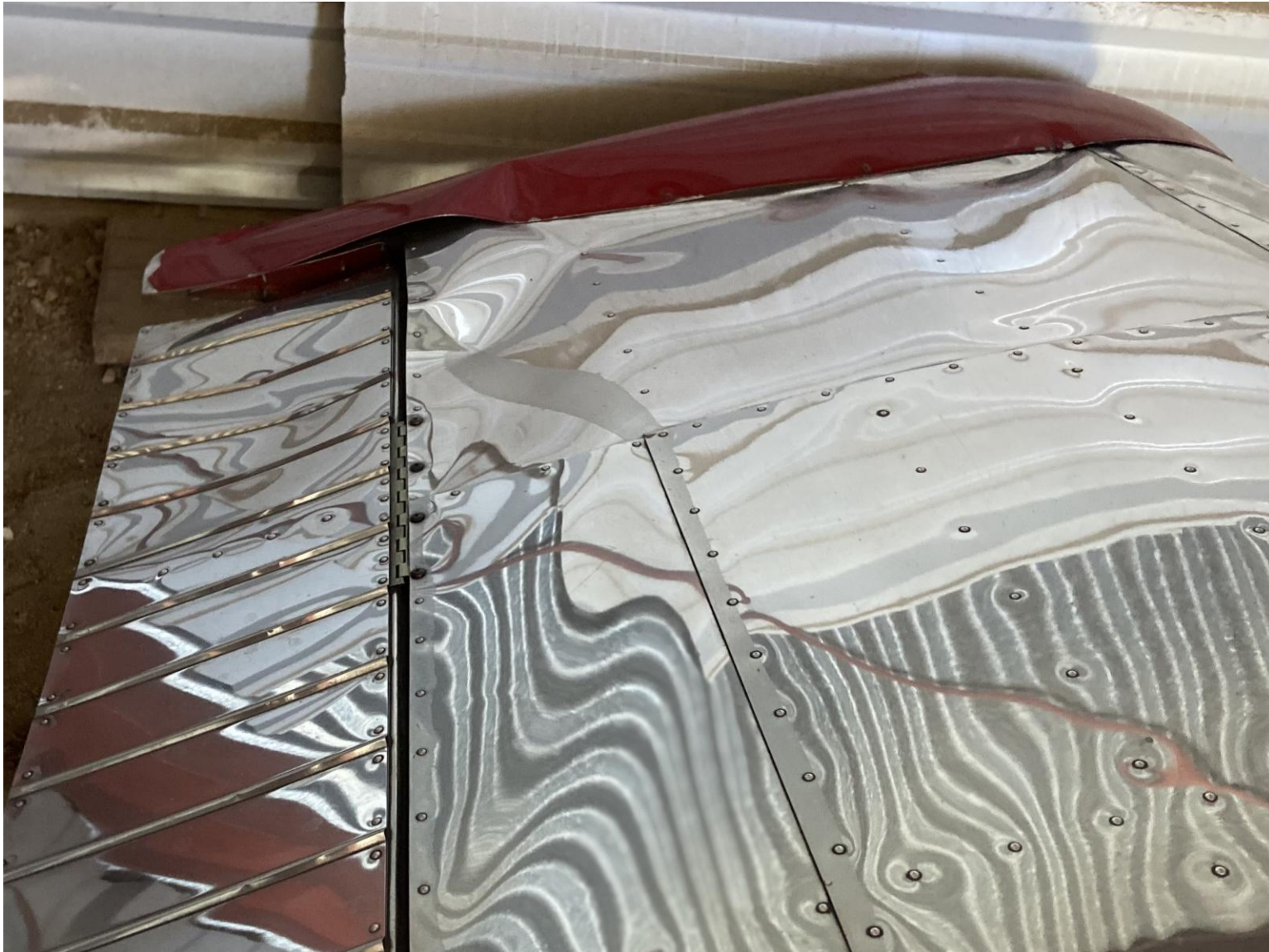
Photograph 6 - Left Wing Damage (Courtesy of FAA)
