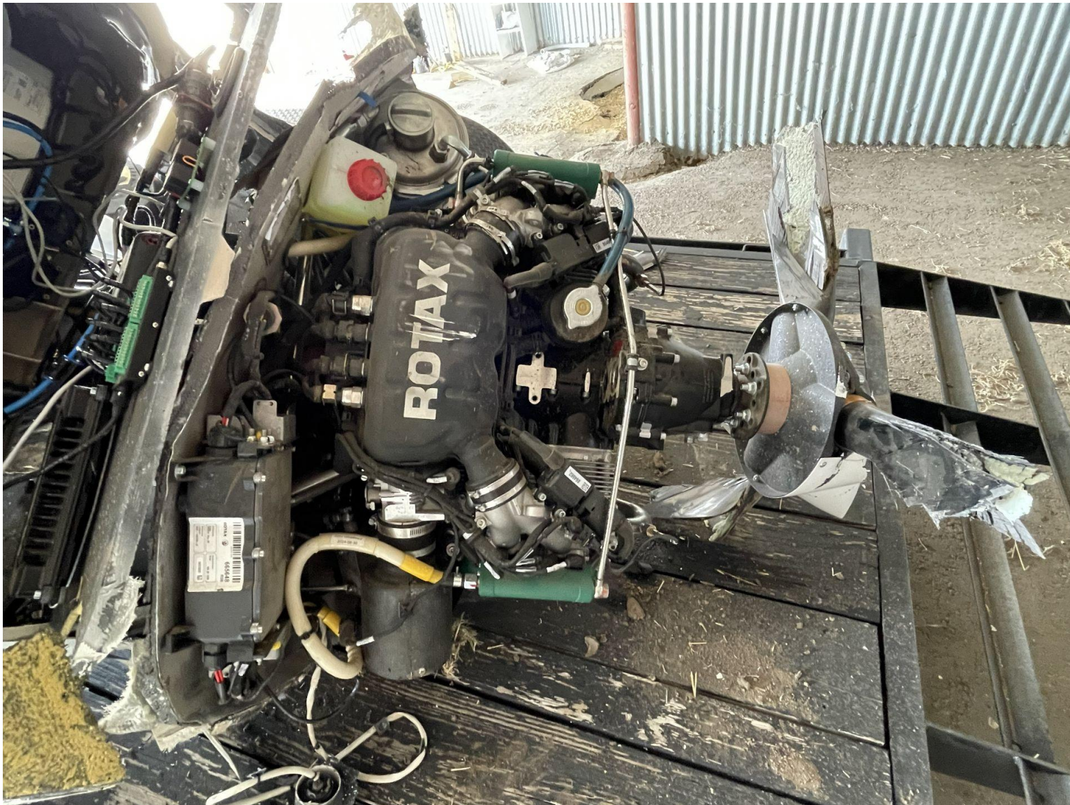
Photograph 8 - Engine / propeller (NTSB photo)
