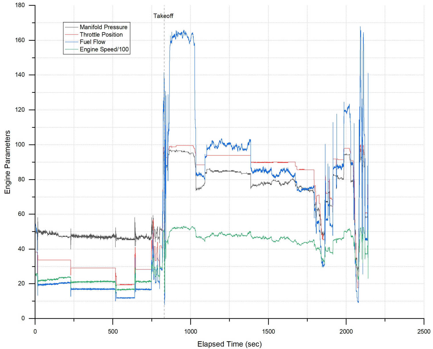
Plot 1 – Basic parameters / Entire flight
