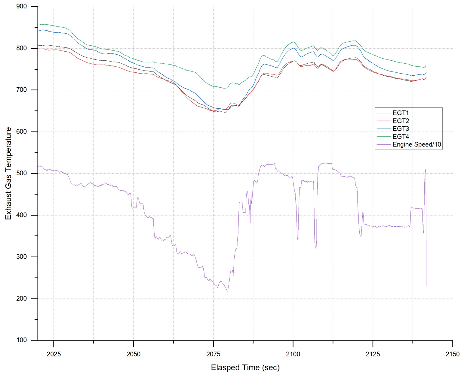
Plot 6 – Exhaust gas temperatures / Final 2-minute flight segment
