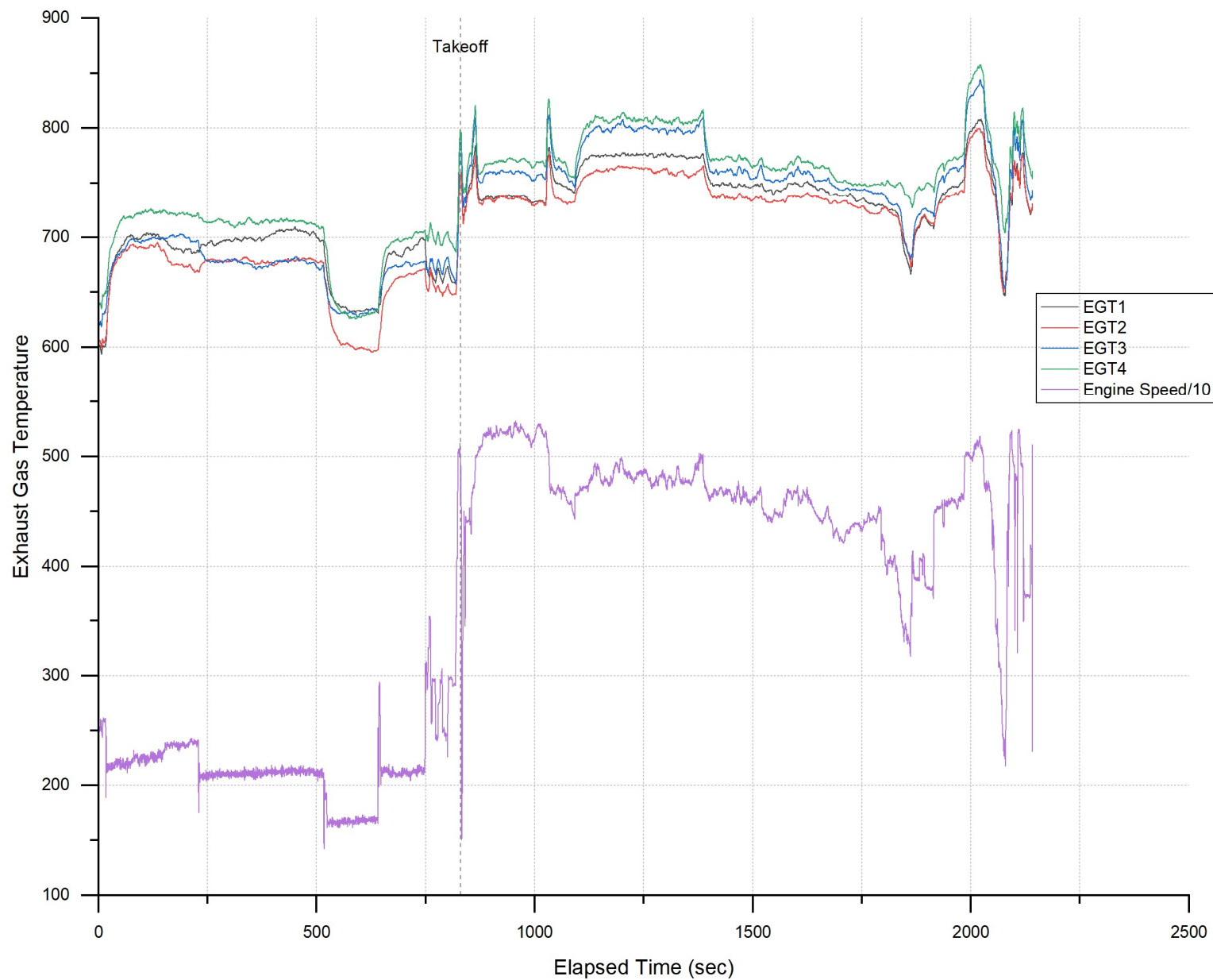
Plot 5 - Exhaust Gas Temperatures / Entire flight
