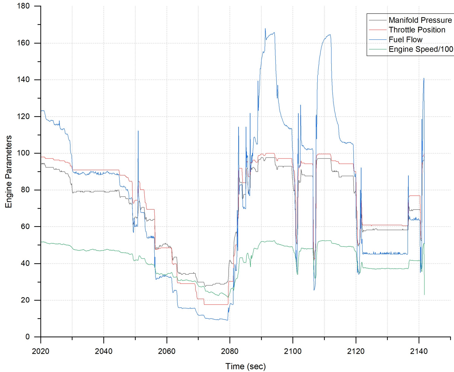
Plot 2 – Basic parameters / Final 2-minute segment
