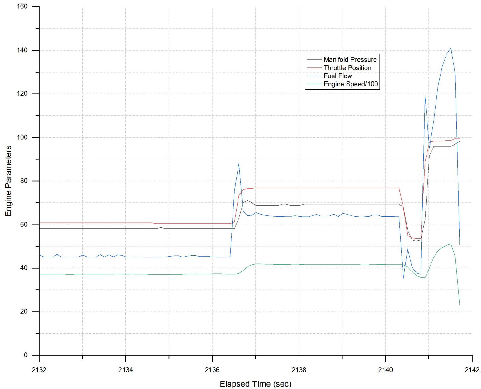
Plot 4 – Basic parameters / Final 10-second flight segment
