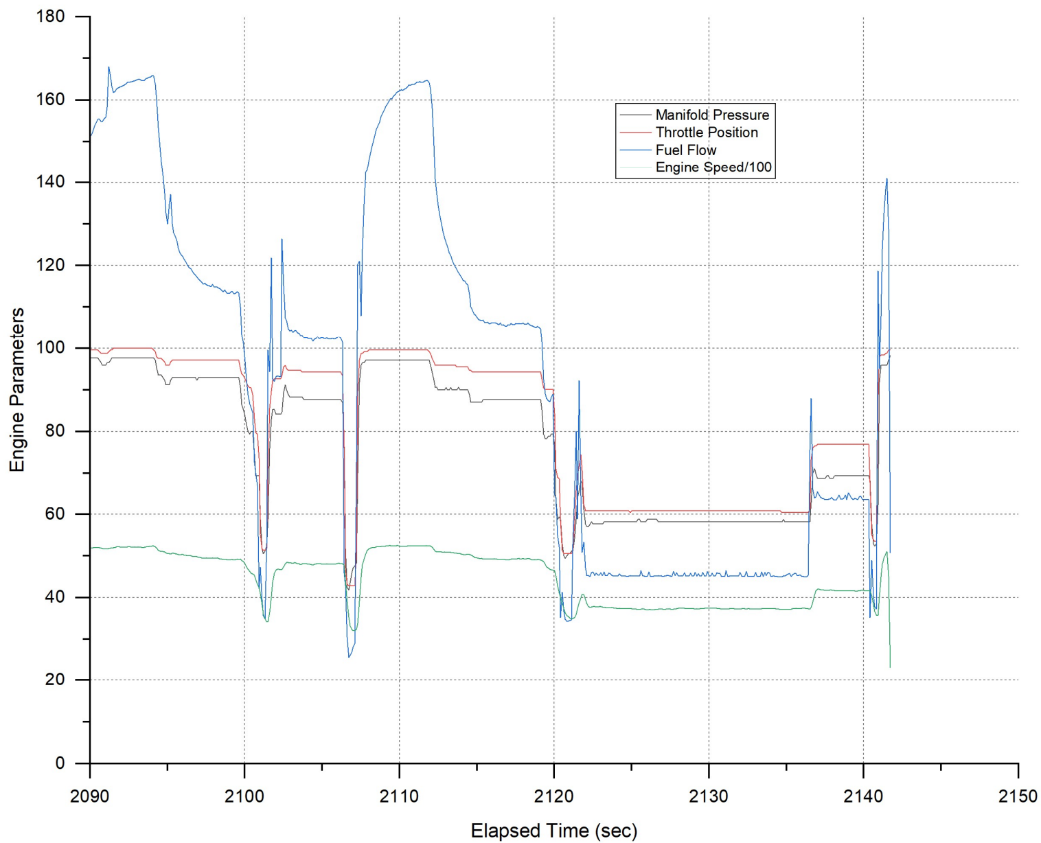
Plot 3 – Basic parameters / Final 1-minute flight segment
