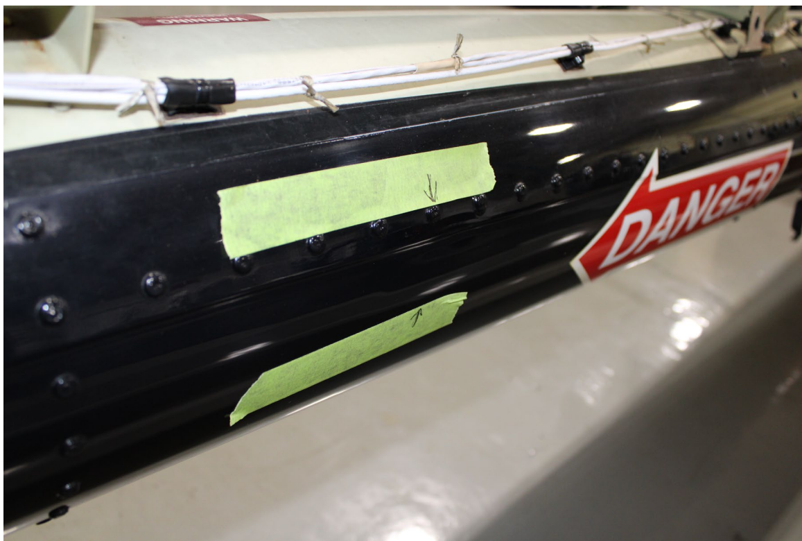
Photograph 1 - Damage to Tailboom (Courtesy of Repair Facility)
