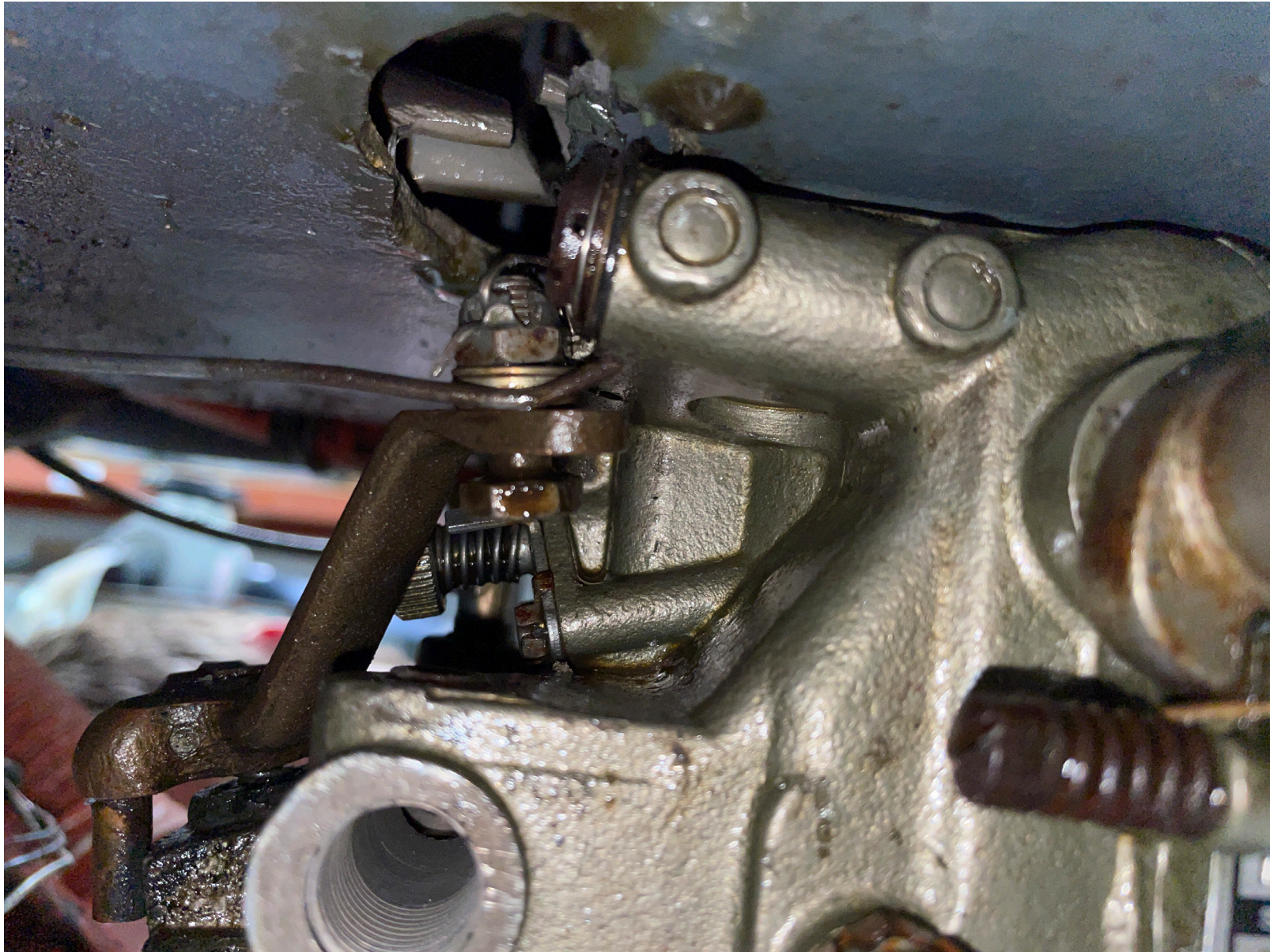
Photograph 7 - Mixture control cable and carburetor (Courtesy of NTSB)
