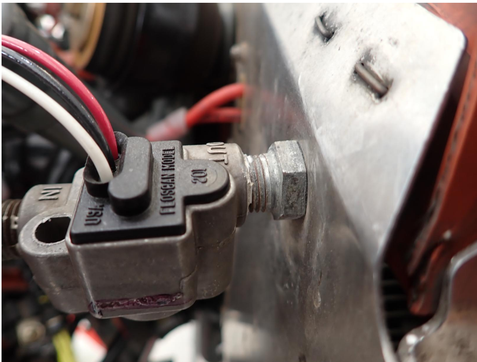
Photograph 2 - Fuel Flow Transducer Attachment Fittings
