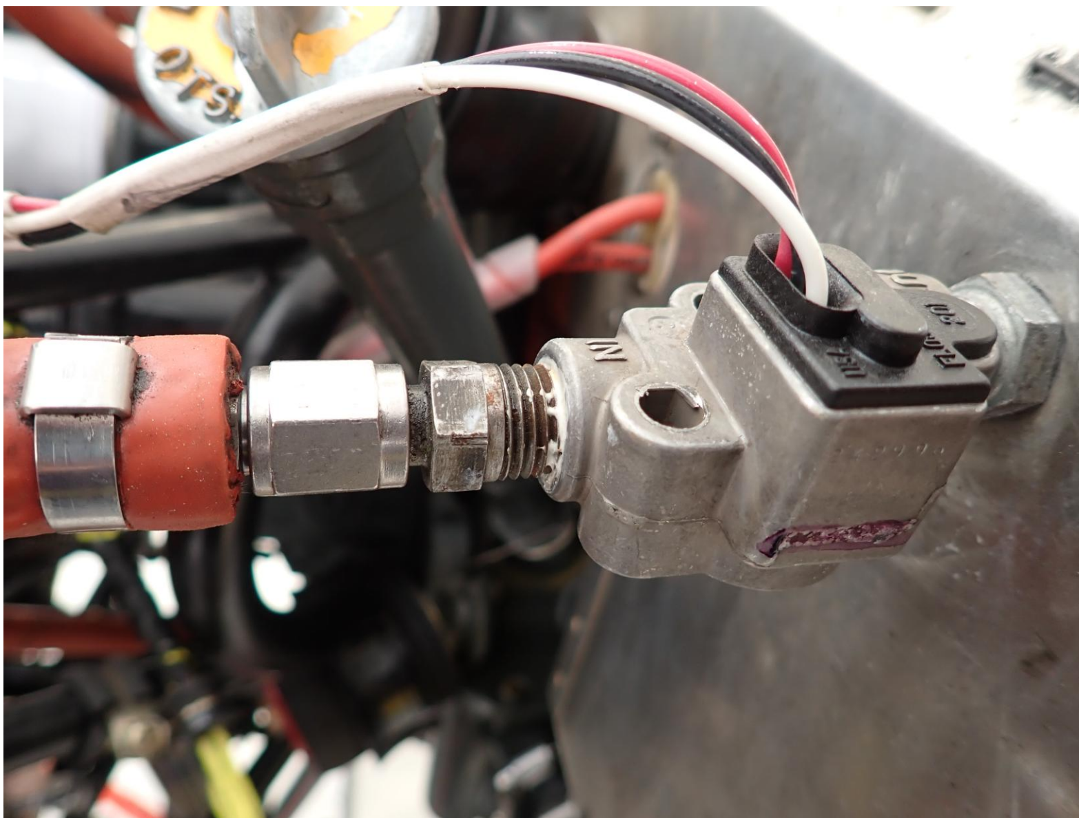
Photograph 3 - Fuel Flow Transducer Attachment Fittings
