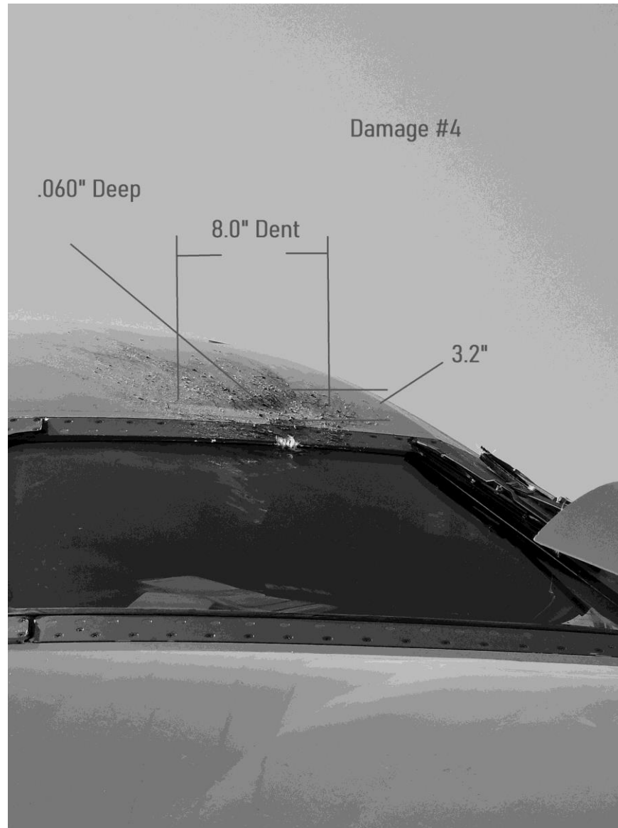
Photograph 5 - Right Side Windshield (Operator Photo)
