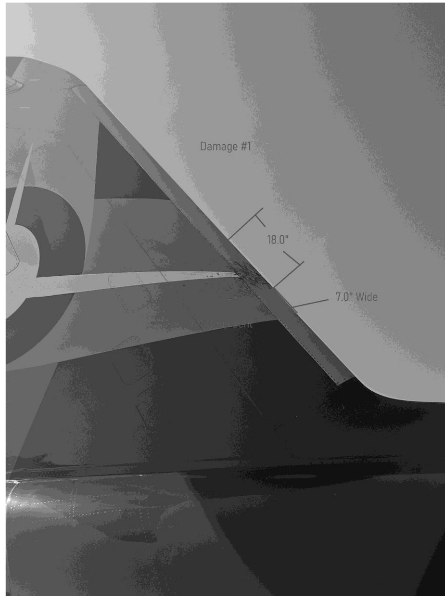
Photograph 6 - Vertical Stabilizer (Operator Photo)
