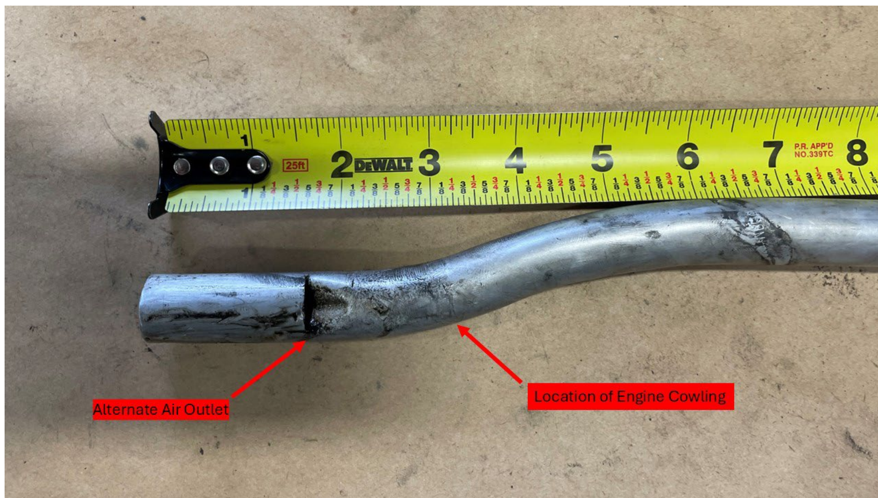
Photograph 4 - Engine oil breather tube with alternate air outlet and location of engine cowling
