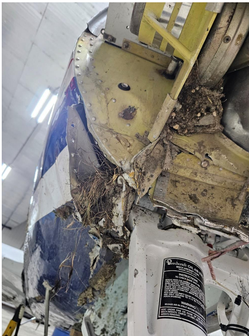
Photograph 7 - Fuselage (Park Rapids Aviation)
