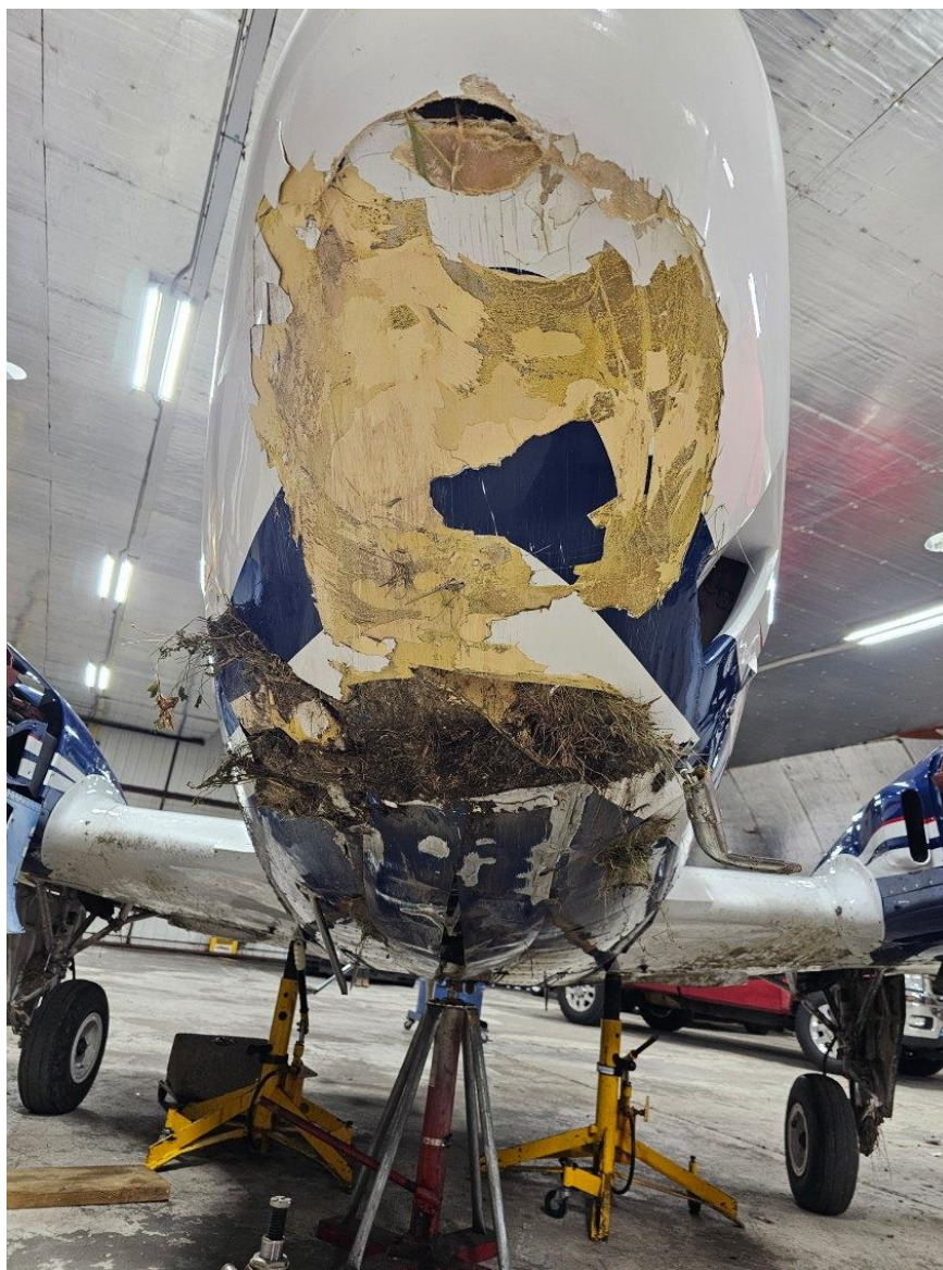
Photograph 2 - Forward Fuselage (Park Rapids Aviation)
