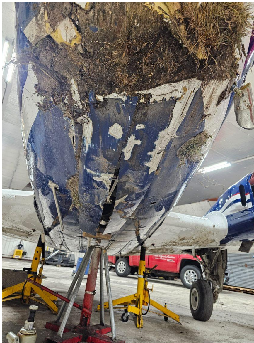
Photograph 3 - Forward Fuselage (Park Rapids Aviation)
