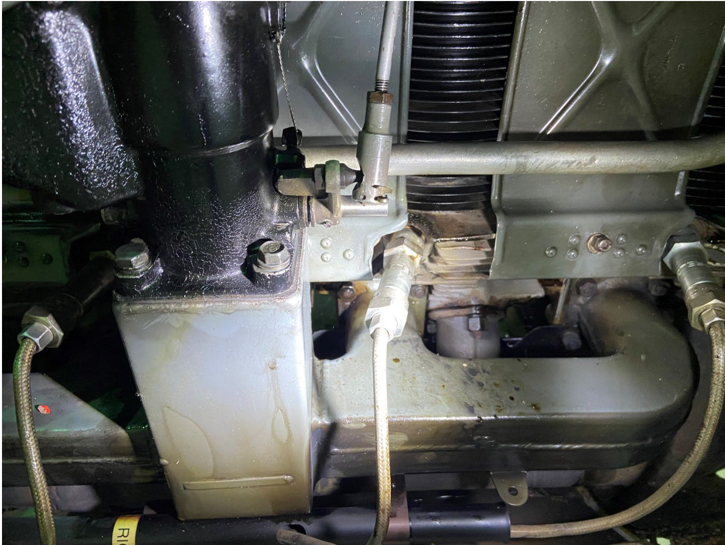
Photograph 5 - Number 4 Cylinder Assembly and Throttle Cable Linkage (Courtesy of Federal Aviation Administration)
