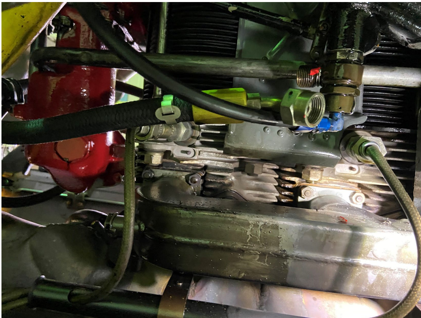
Photograph 4 - Number 2 Cylinder Assembly (Courtesy of Federal Aviation Administration)
