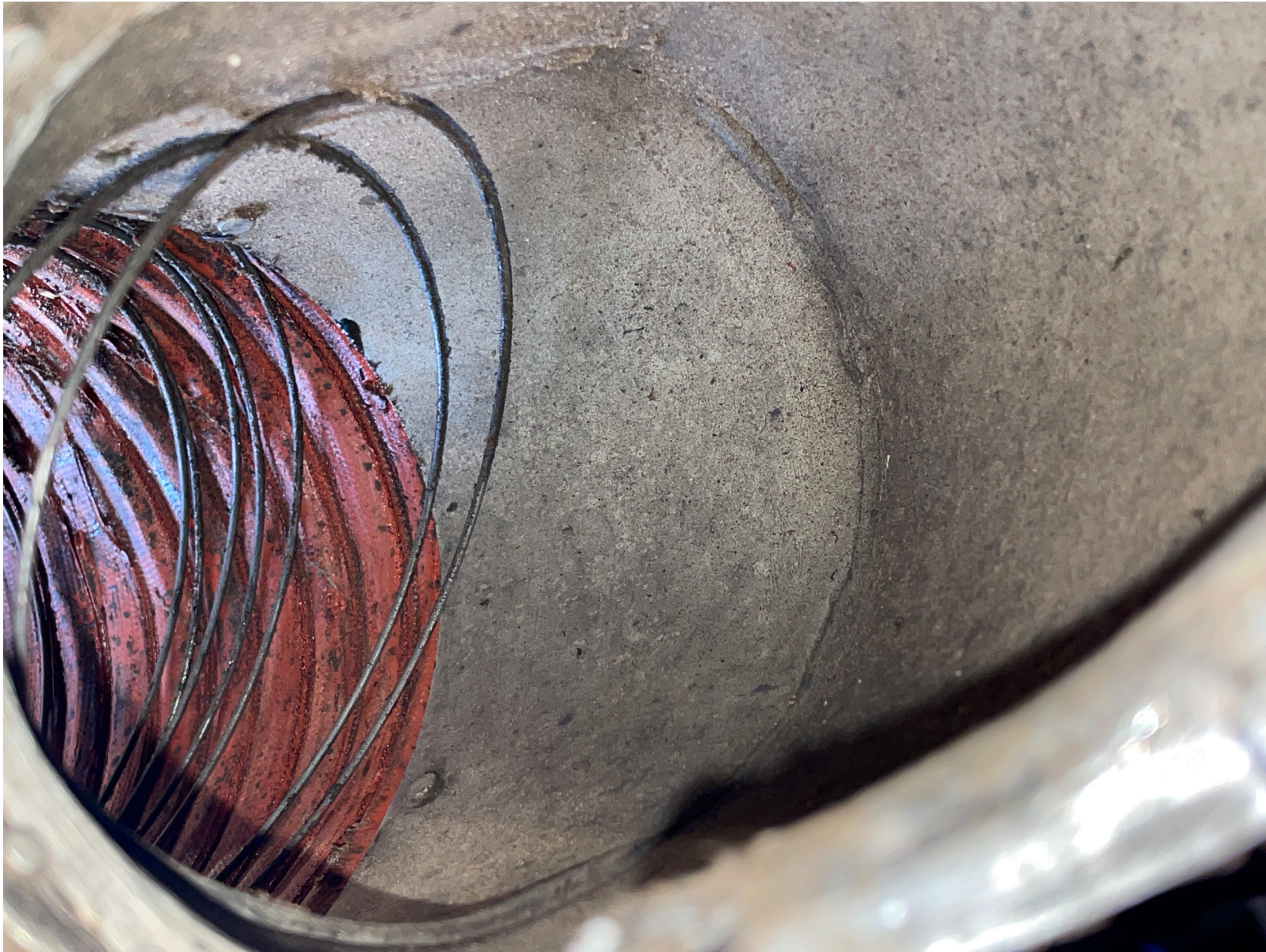
Photograph 8 - Collapsed and degraded scat duct (Courtesy of NTSB)
