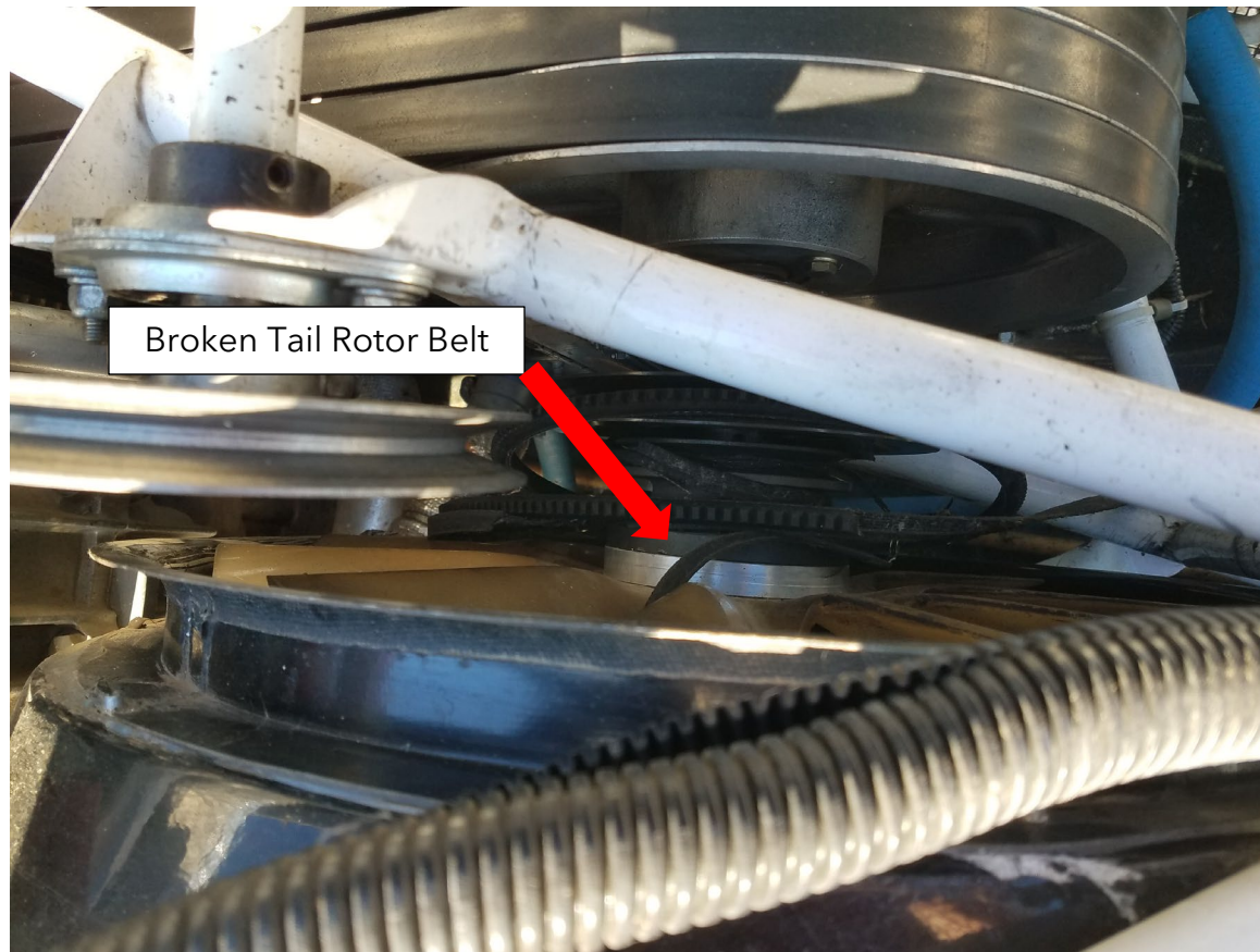
Photograph 2 - Broken tail rotor belt (Courtesy of Owner)
