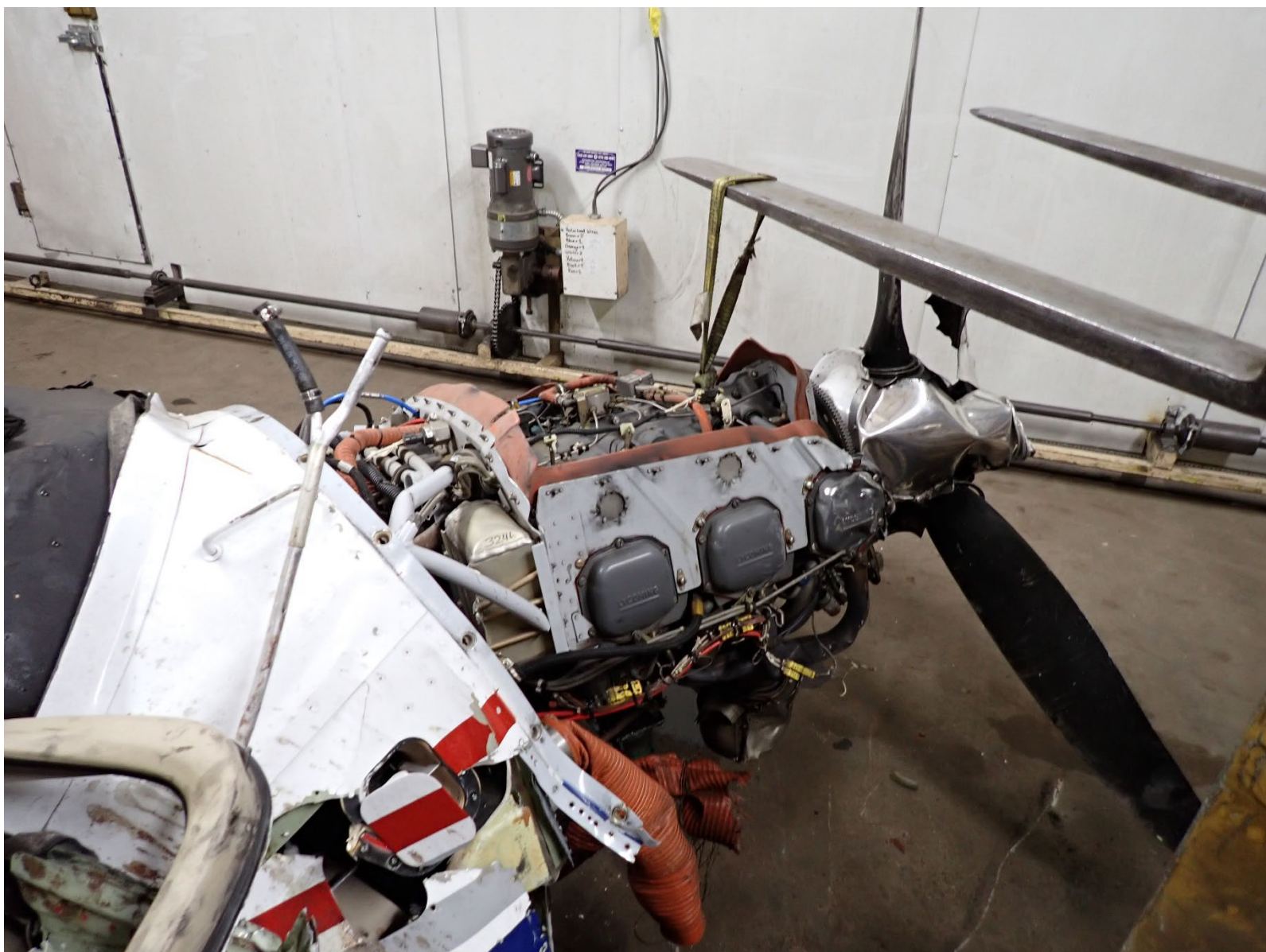
Photograph 4 - Engine, Right Side (Courtesy of Textron Aviation)
