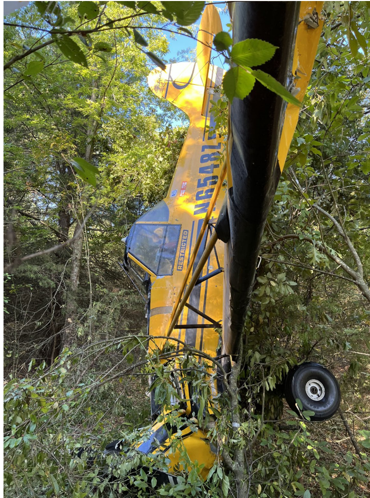
Photograph 1 - Fuselage damage (Courtesy of FAA)
