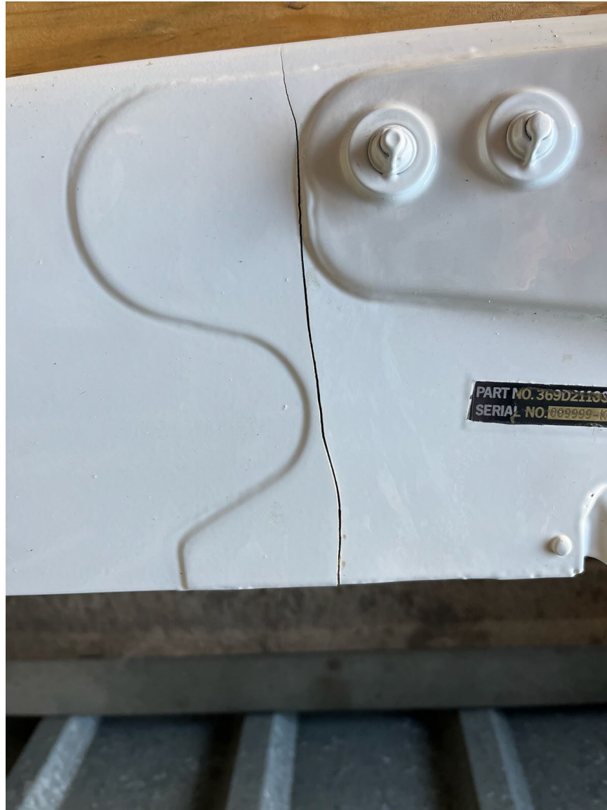
Photograph 3 - View of the substantial damage on the bottom of the main rotor blade (courtesy of the Federal Aviation Administration)
