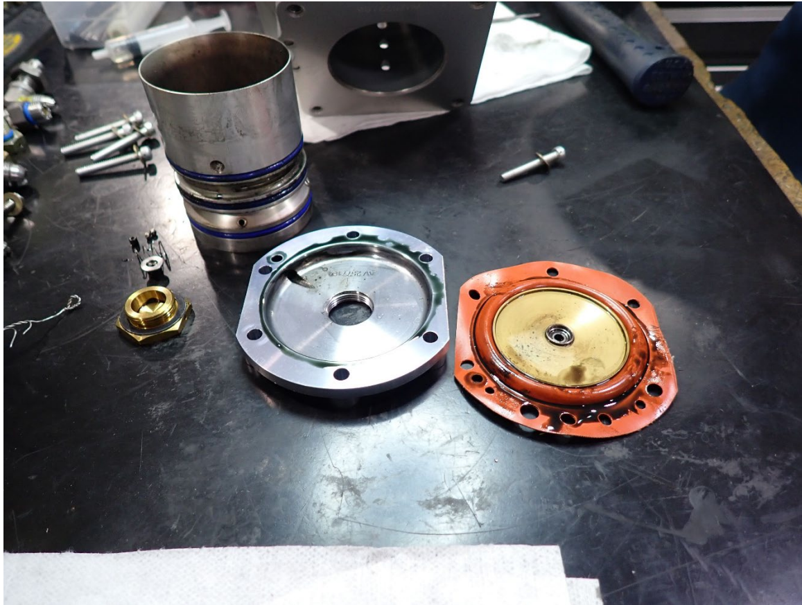
Photograph 2 - Venturi and Air Diaphragm (Courtesy of FAA)
