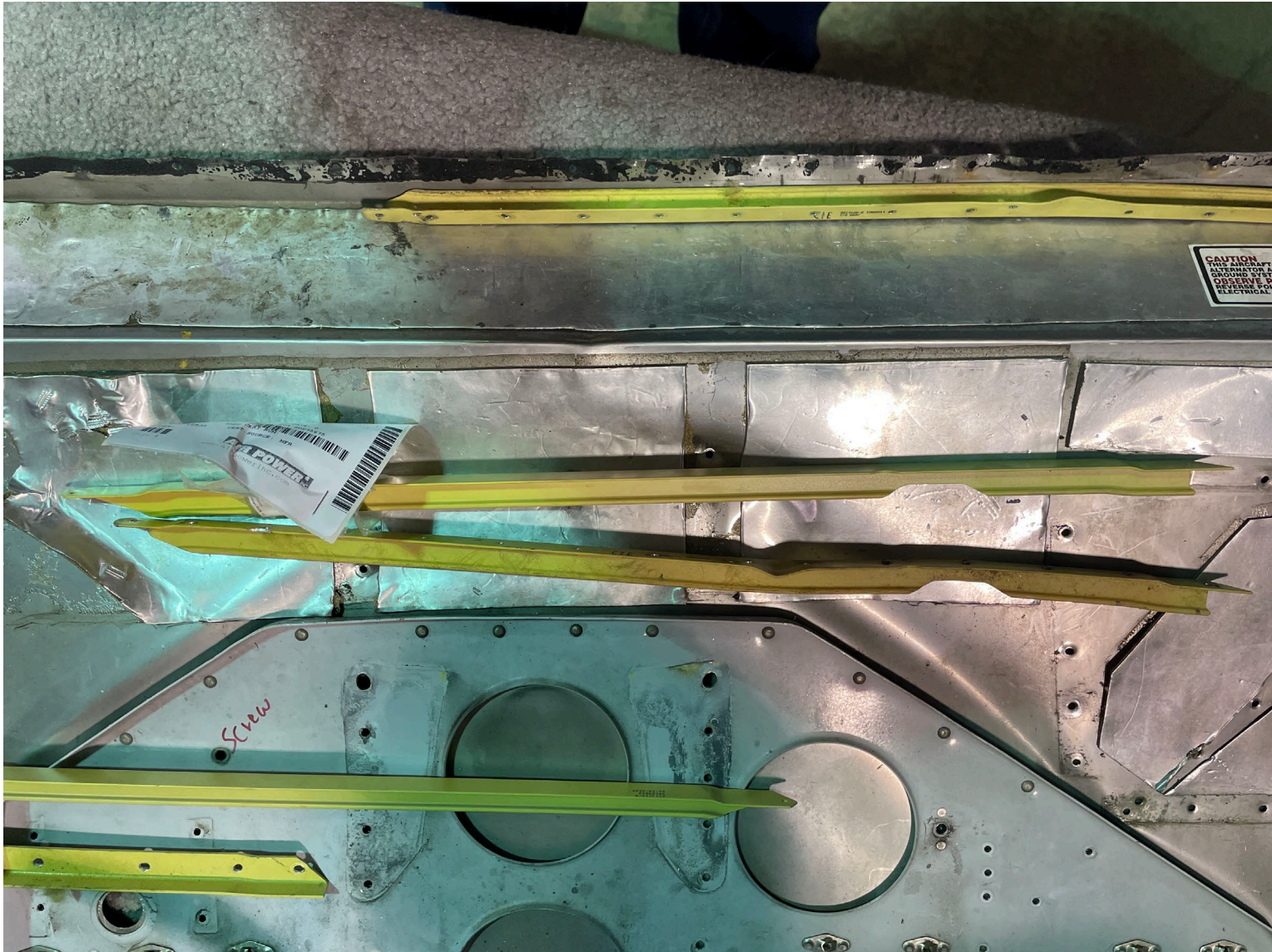
Photograph 2 - Bent Stringers (Courtesy of Federal Aviation Administration)
