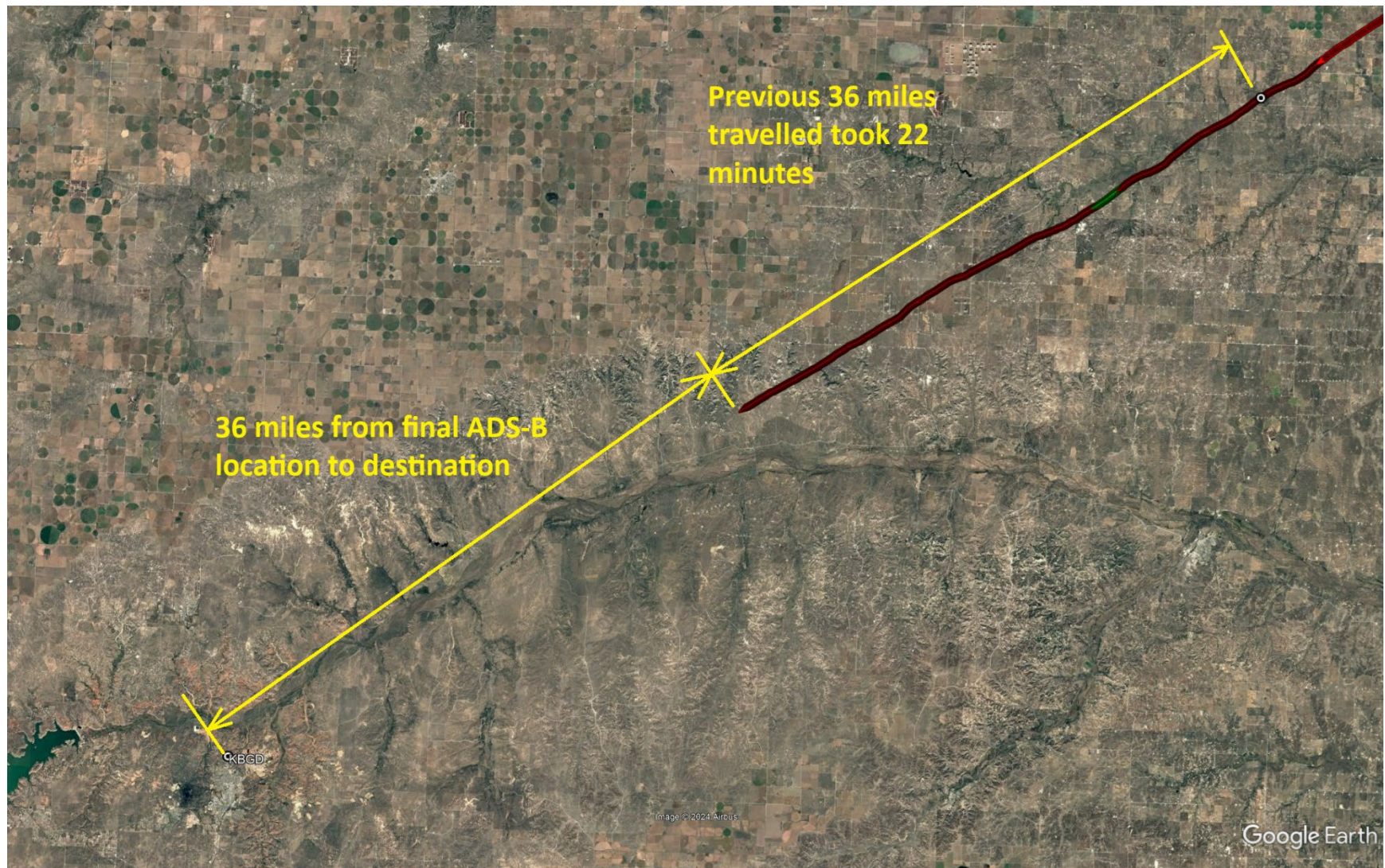
Figure 2 – Plot of the final portion of the accident flight path.
