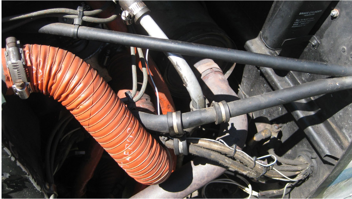
Photograph 2 - Bent engine mount (Courtesy of FAA)
