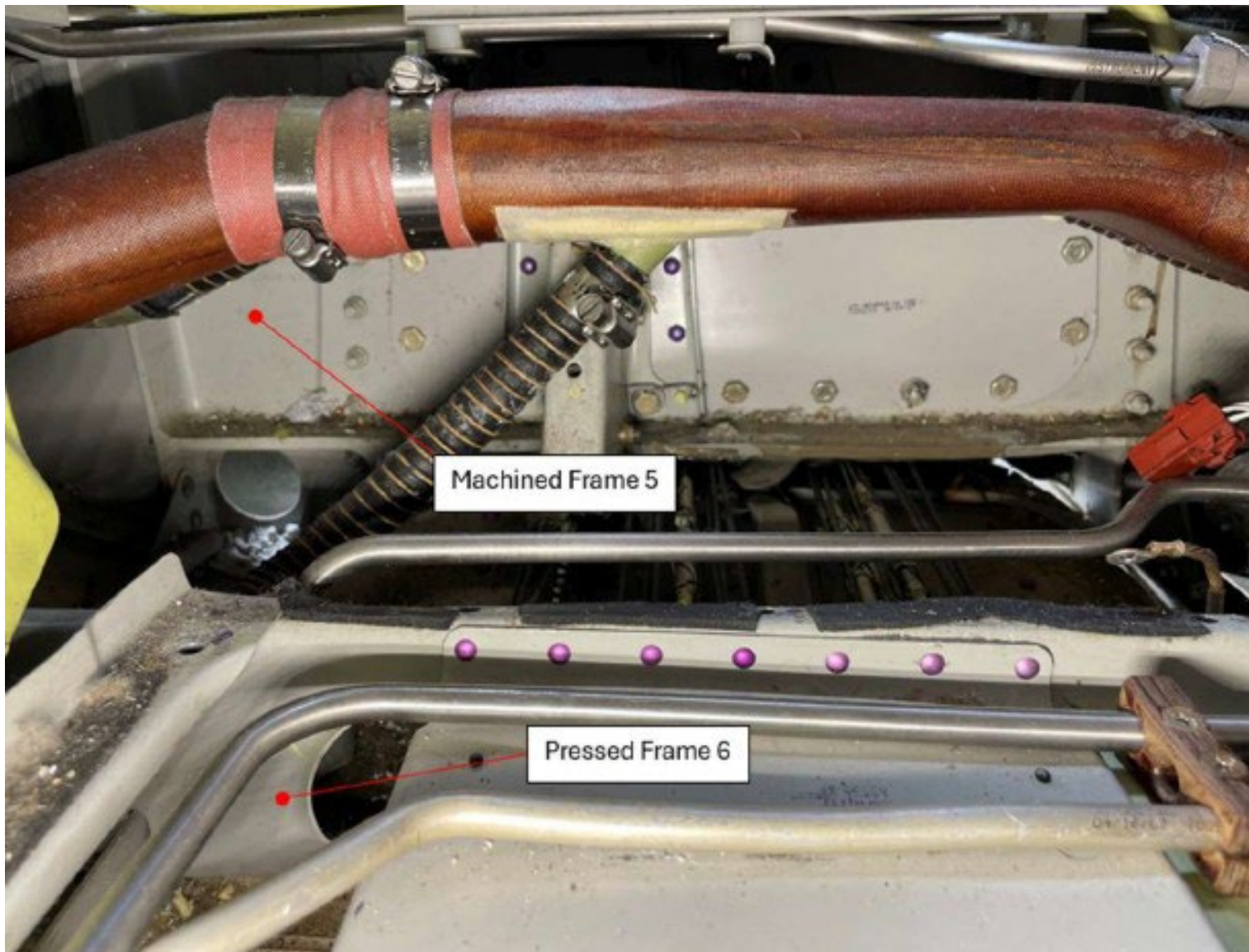
Photograph 10 - View of the substantial deformation damage sustained to the frame 5 lower assembly and the lower frame 6 pressing (courtesy of Textron Aviation)
