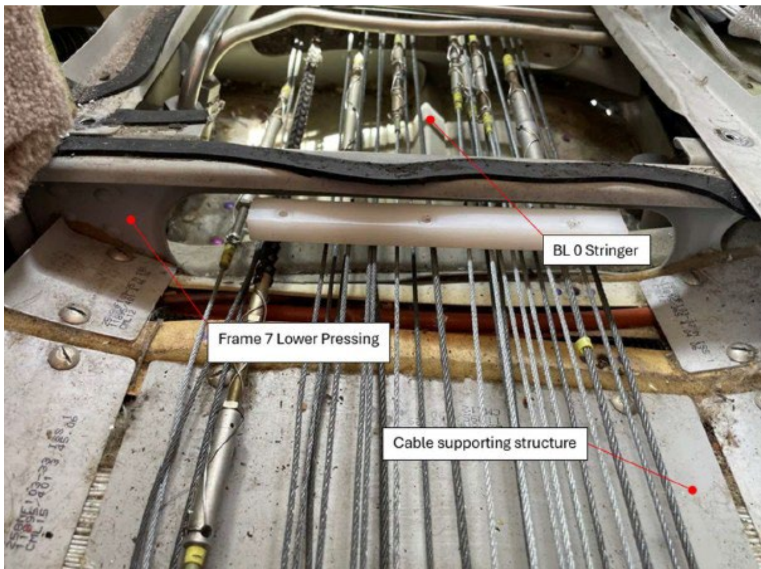
Photograph 11 - View of the substantial deformation damage sustained to the frame 7 lower assembly (courtesy of Textron Aviation)
