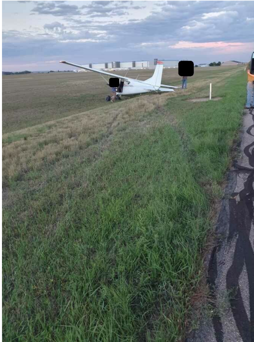
Photograph 3 - View of the rear of the airplane at the accident site (courtesy of the pilot)
