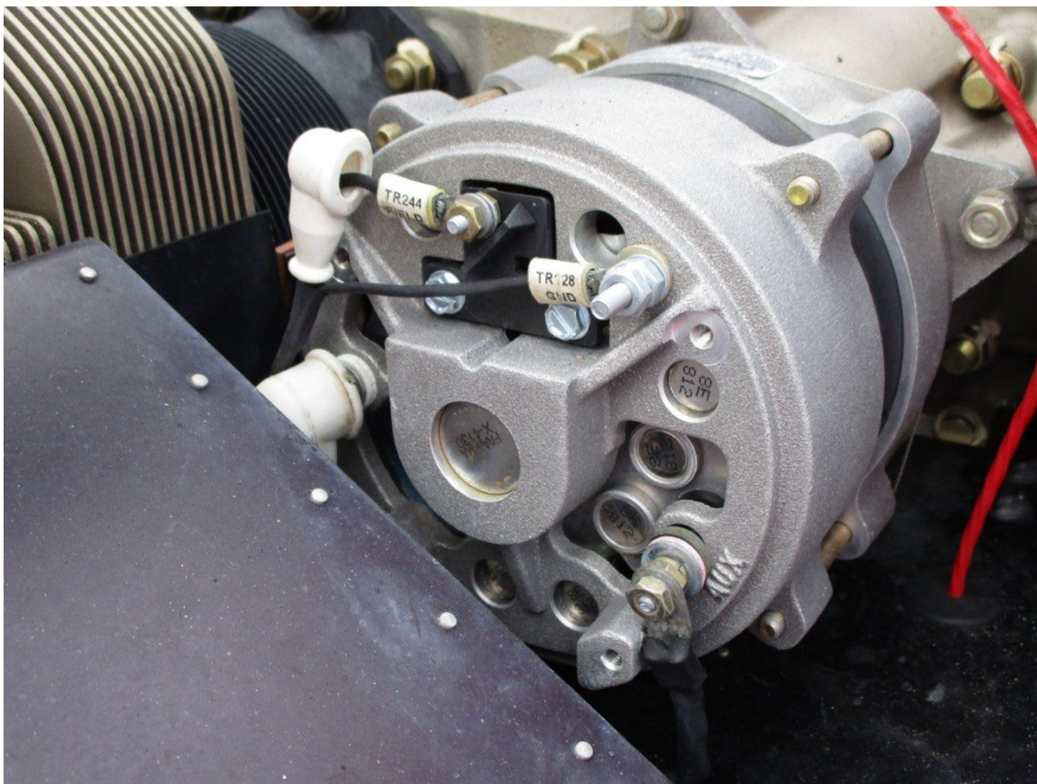
Photograph 1 - Alternator Installation at Time of the Accident (Courtesy of the Federal Aviation Administration)
