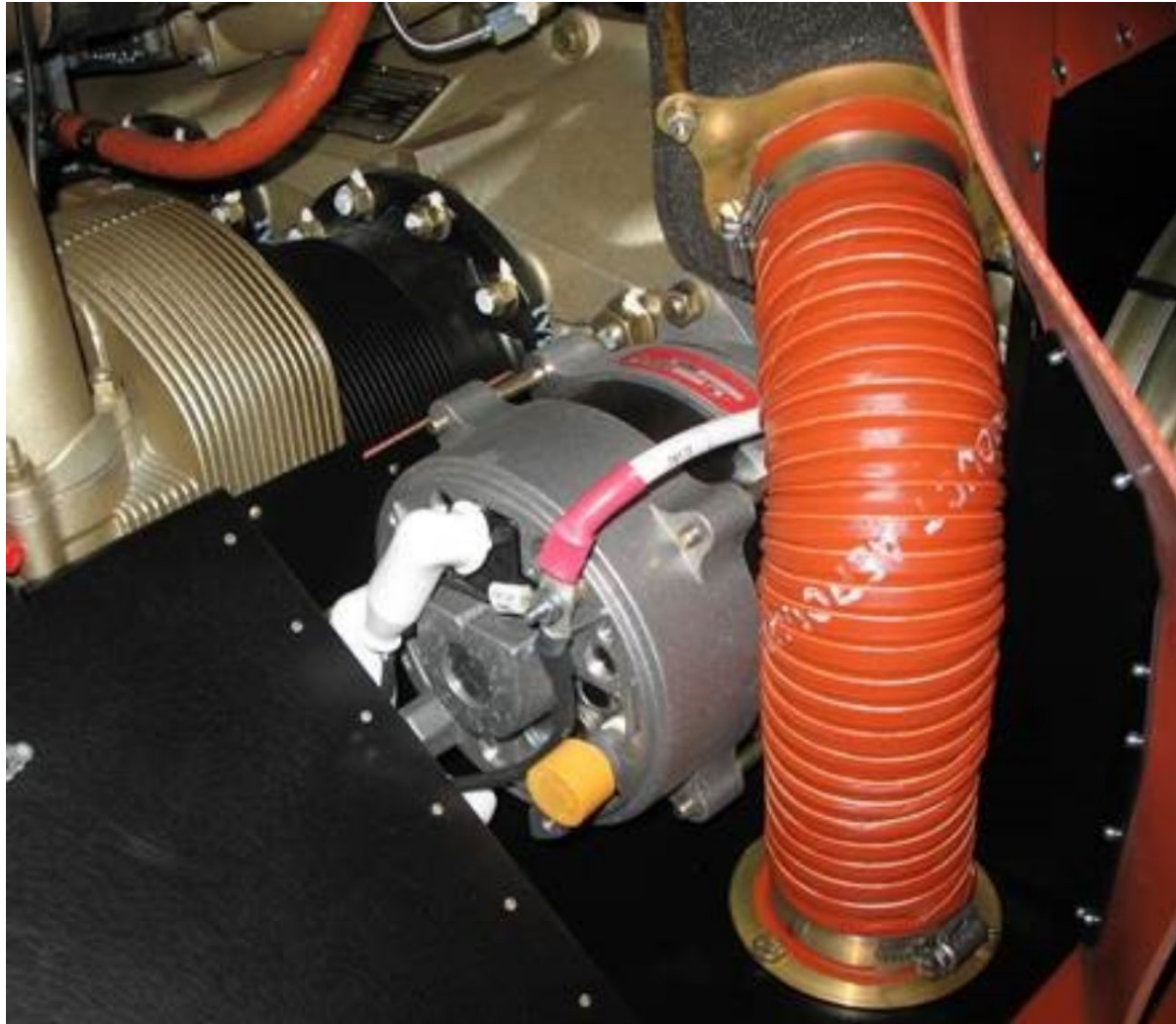
Photograph 2 - Alternator Installation in Accordance with the Cirrus Maintenance Manual Models SR22 and SR22T (Courtesy of Cirrus Aircraft)
