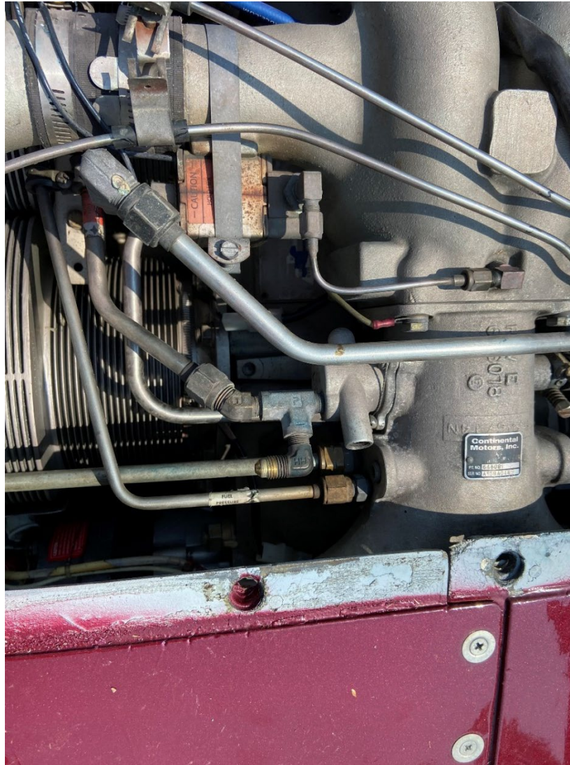
Photograph 4 - View of the metered pressure test fitting at the accident site, with the protective cap not installed and blue staining present on the fitting (courtesy of the Federal Aviation Administration)
