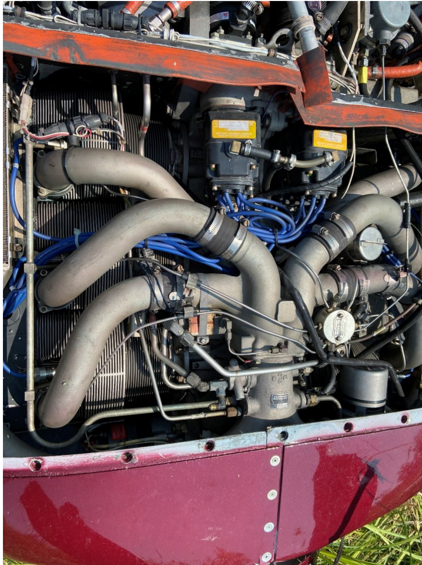
Photograph 3 - View of the engine at the accident site (courtesy of the Federal Aviation Administration)
