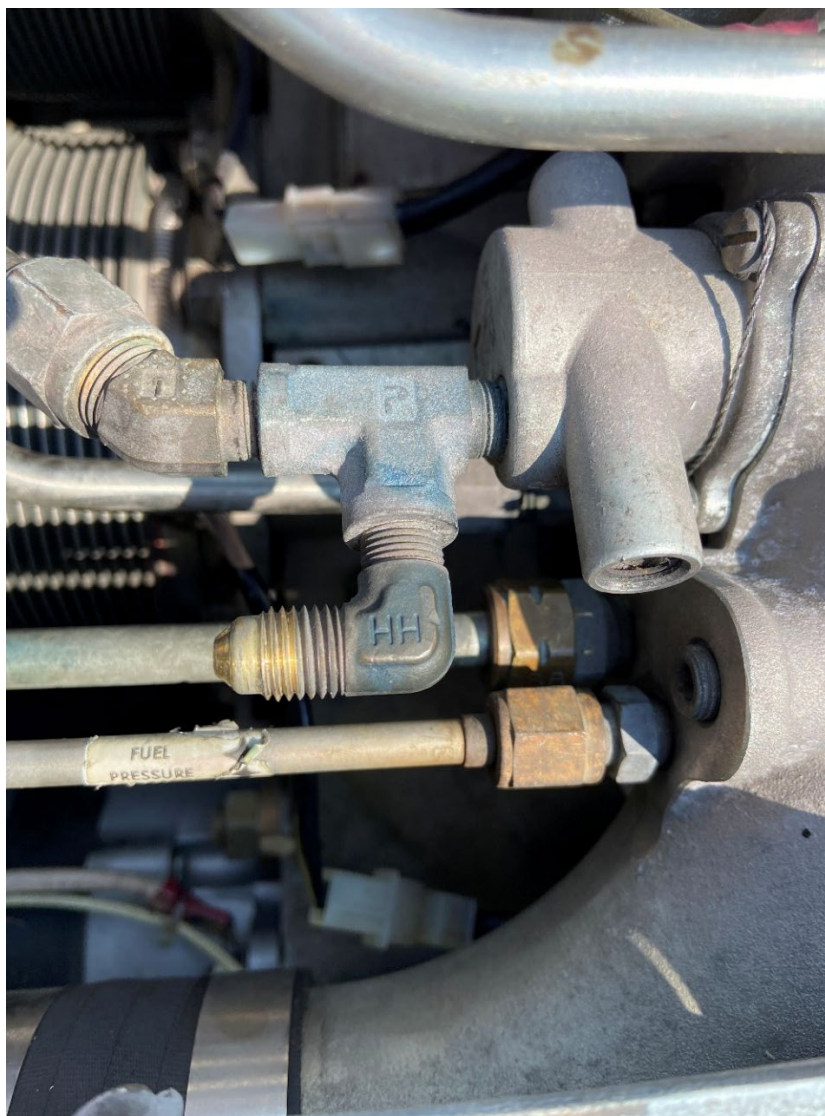
Photograph 5 - View of the metered pressure test fitting at the accident site, with the protective cap not installed and blue staining present on the fitting (courtesy of the Federal Aviation Administration)
