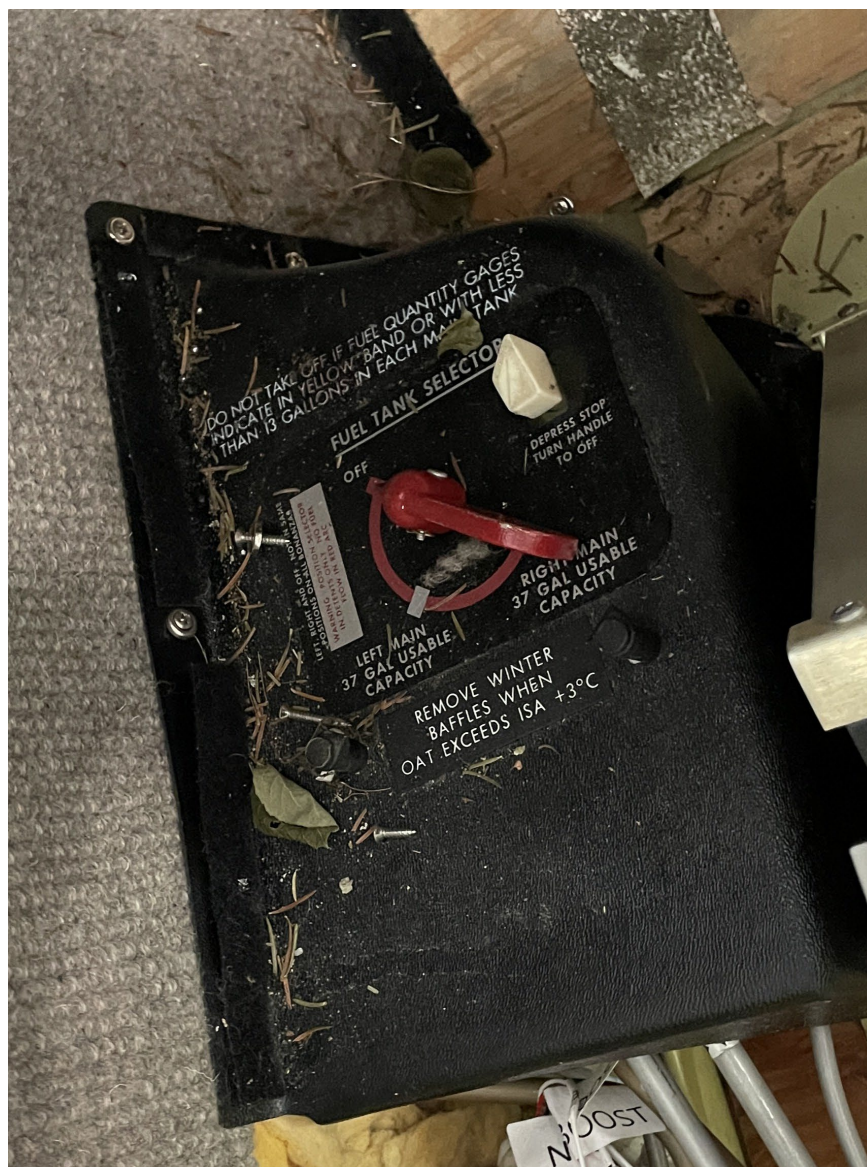
Photograph 3 - Fuel Selector and Placard (Courtesy of NTSB)
