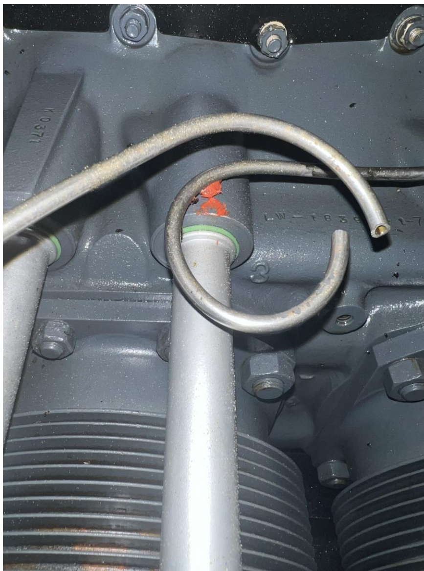
Photograph 7 - Engine Oil Pressure Line (Pilot Photo)
