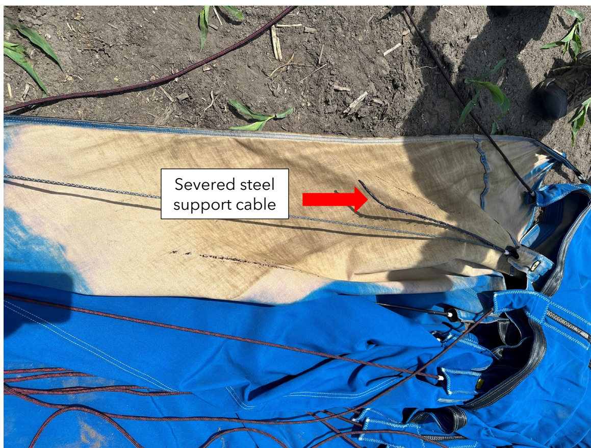
Photograph 2 - Severed steel support cable (Courtesy of FAA)
