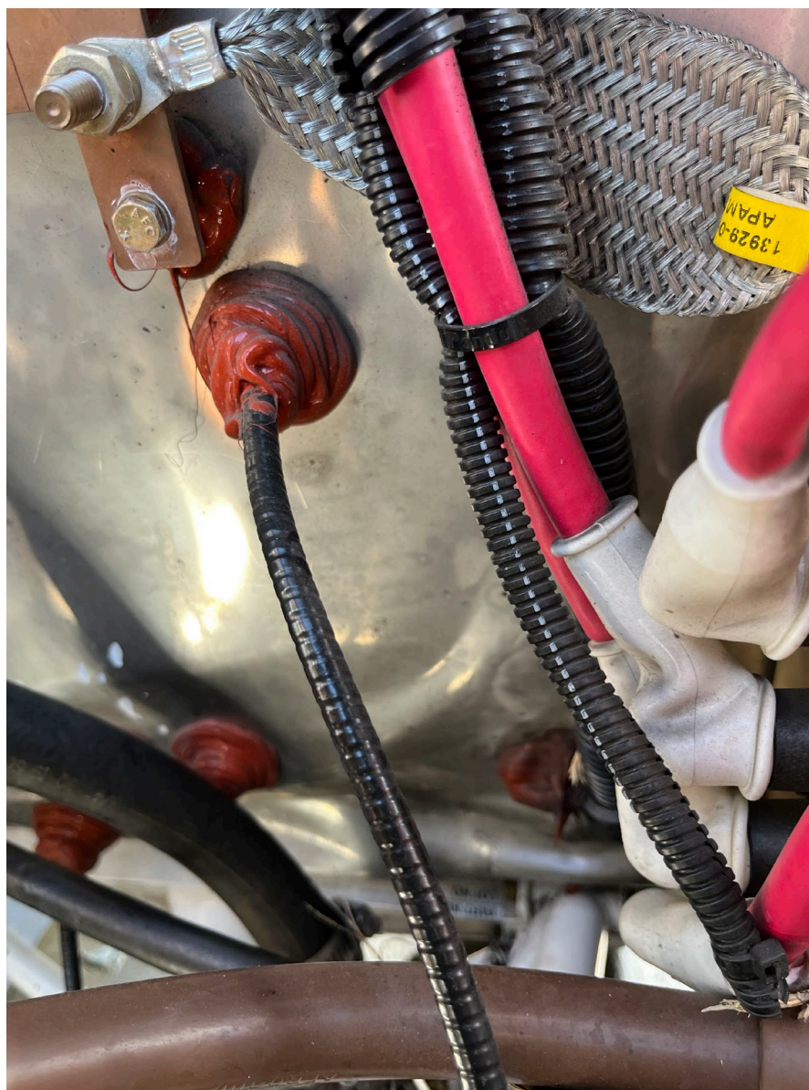
Photograph 3 - Substantial Engine Firewall Damage (Courtesy of FAA)
