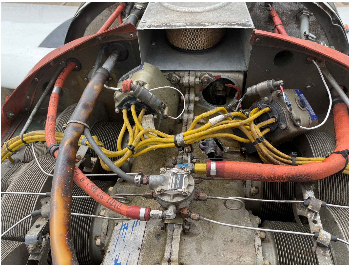
Photograph 1 - Engine (Courtesy of FAA)
