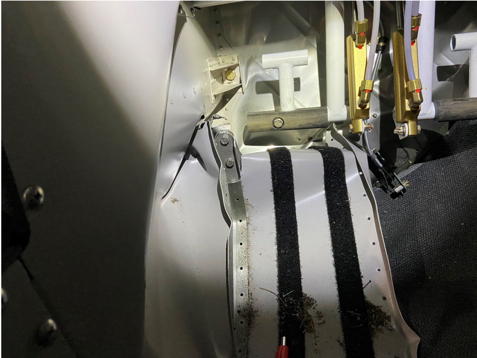
Photograph 6 - View of the substantial damage sustained to the right side cockpit floor (courtesy of the Federal Aviation Administration).
