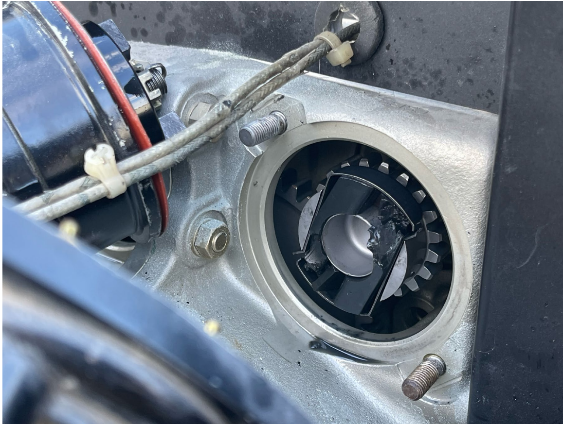
Photograph 4 - Left Magneto & P-Lead Damage (Courtesy of Pilot)
