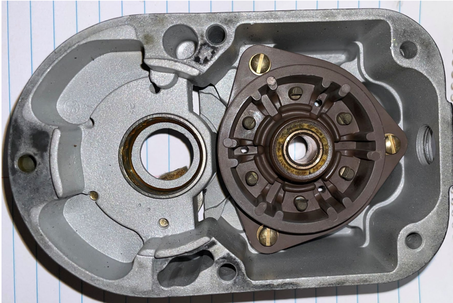
Photograph 4 - Right magneto distributor block Note arcing damage to electrodes and oil saturated felt in the center of the distributor. (Courtesy of NTSB)
