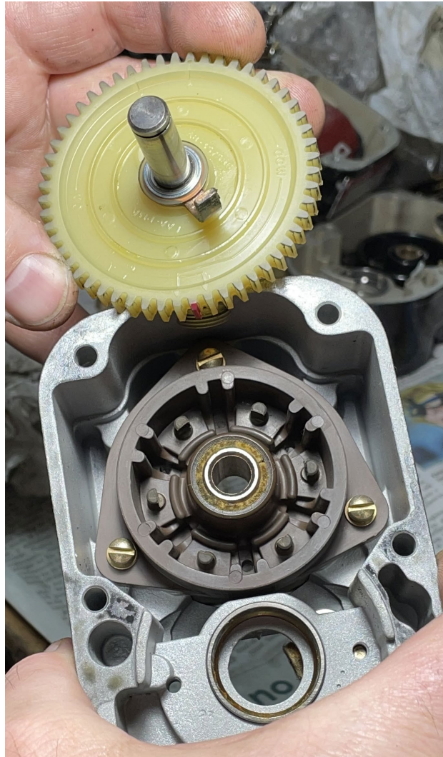
Photograph 3 - Left magneto distributor block and rotor. Note arcing damage to electrodes and oil saturated felt in the center of the distributor. (Courtesy of NTSB)
