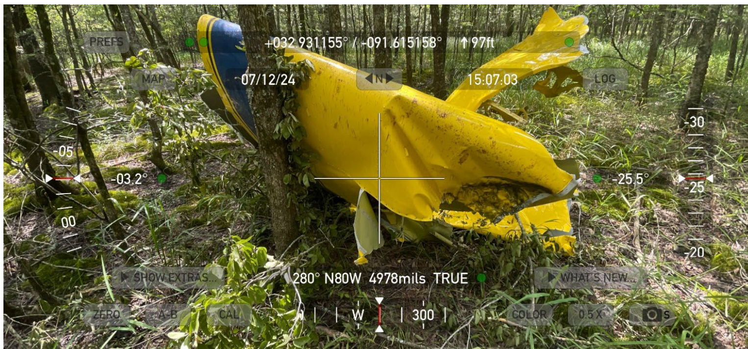
Photograph 8. N6177J Separated outboard left wing (Source: FAA)
