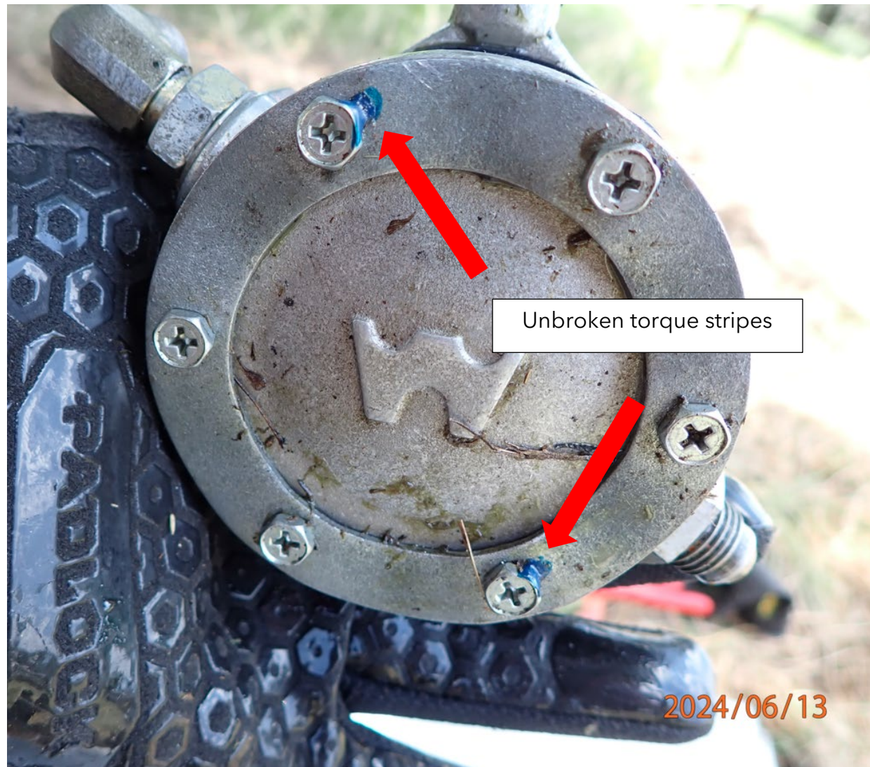
Photograph 11. Bottom of engine driven fuel pump
