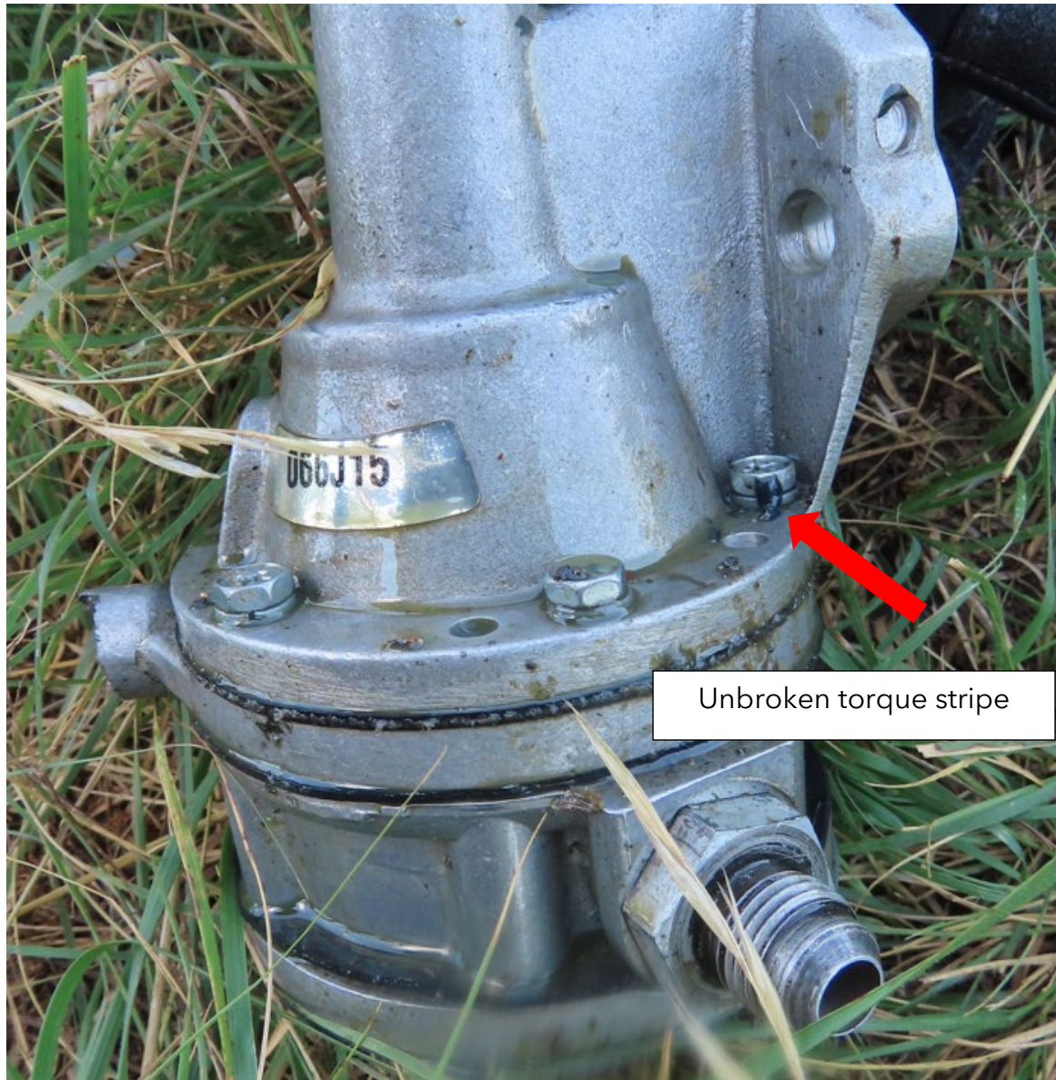
Photograph 12. Top of engine driven fuel pump
