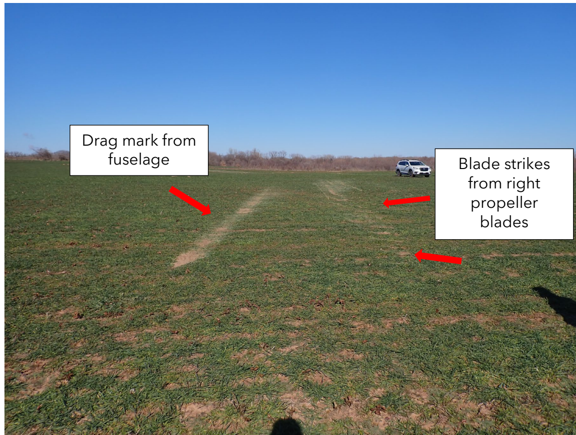
Photograph 1 - Ground Scars
