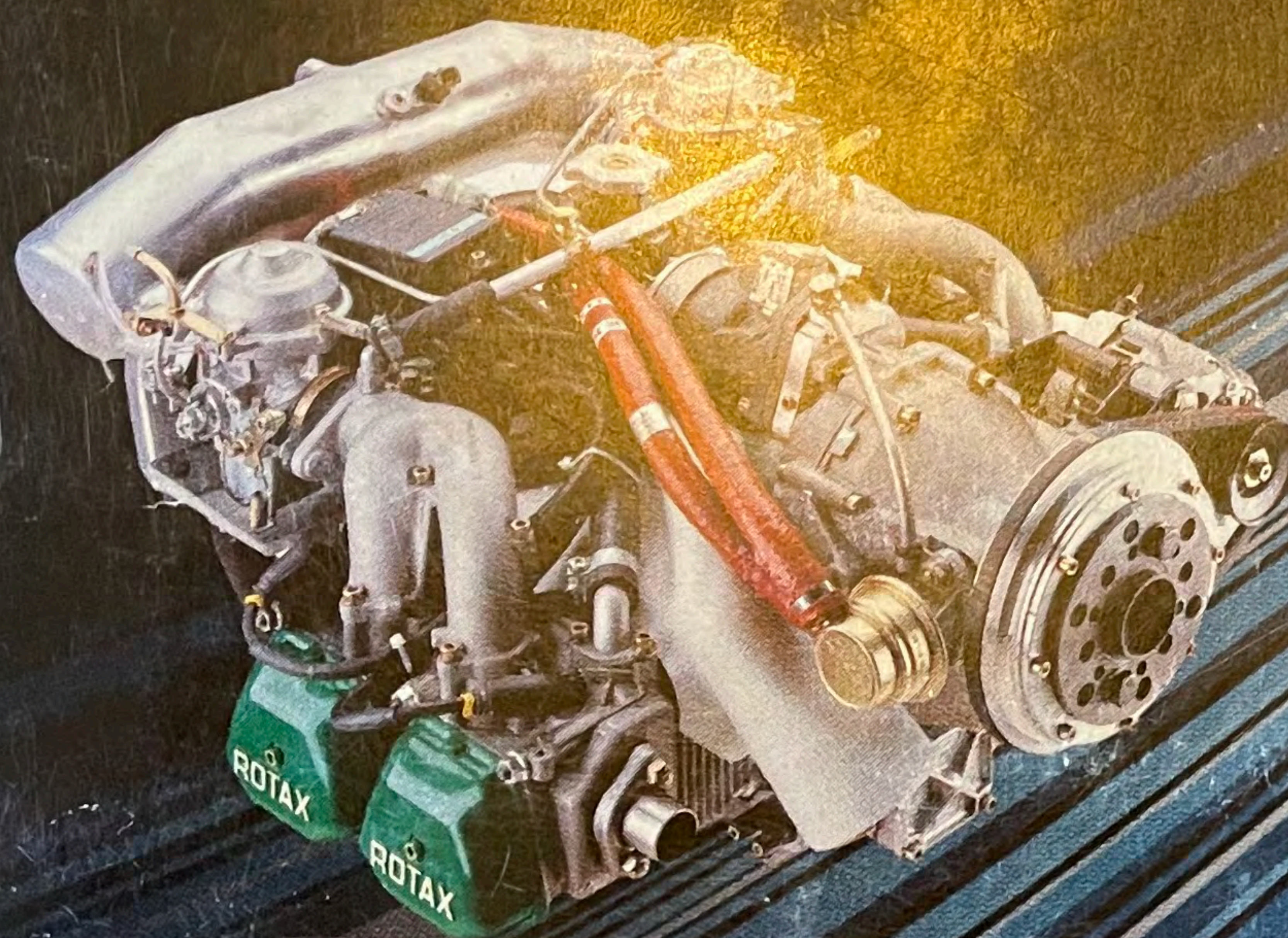
picture ROTAX® 912 ULS 3 with options
