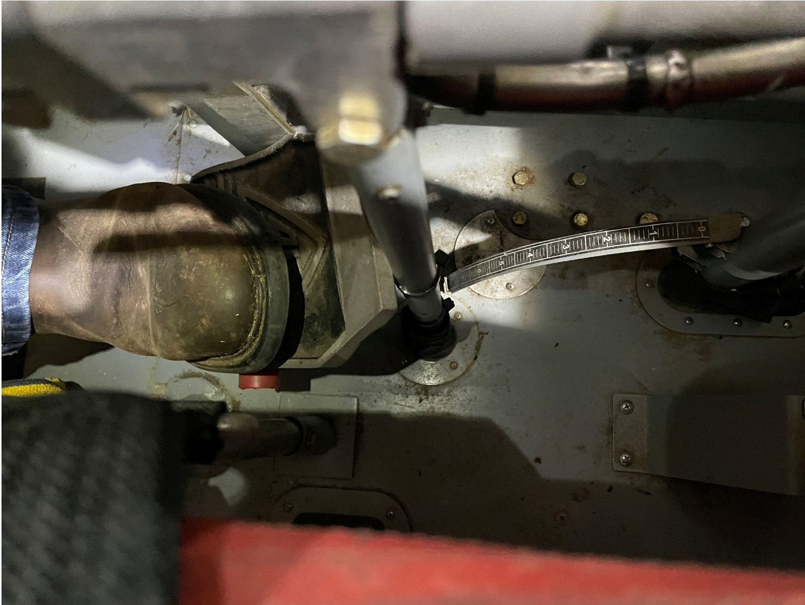
Photograph 7 - Spray valve pushrod and rudder pedal (Courtesy of NTSB)
