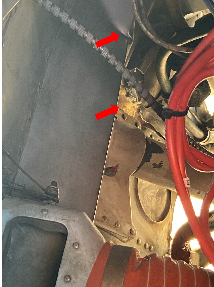
Photograph 1 - Damaged Upper and Lower Firewall (Courtesy of FAA)
