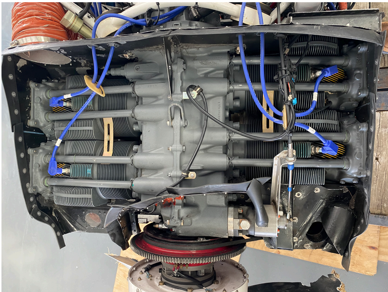
Photograph 7 - Top view of engine (Courtesy of FAA)
