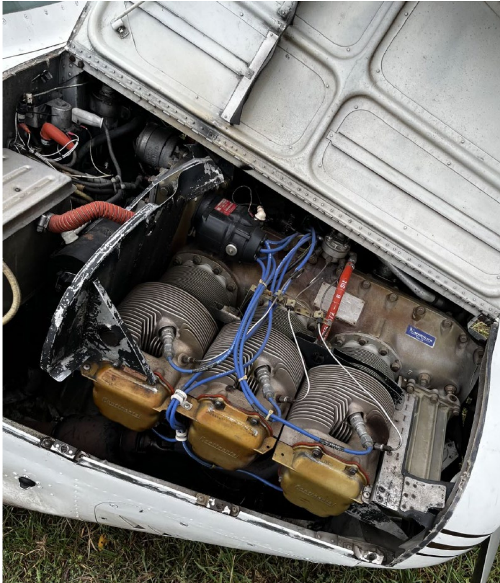
Photograph 6 - View of the right side of the engine at the accident site (courtesy of the Federal Aviation Administration)
