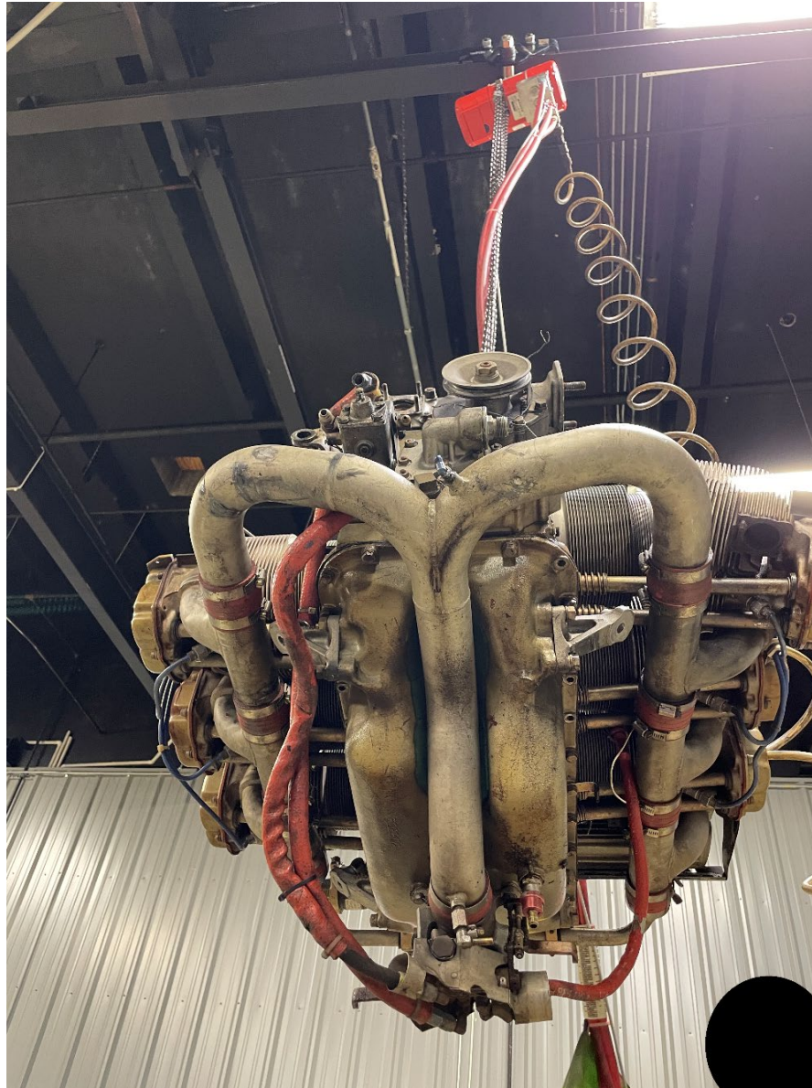
Photograph 10 - View of the bottom of the engine during the engine examination
