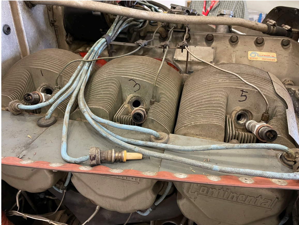
Photograph 6 - Engine during examination (Courtesy of FAA)
