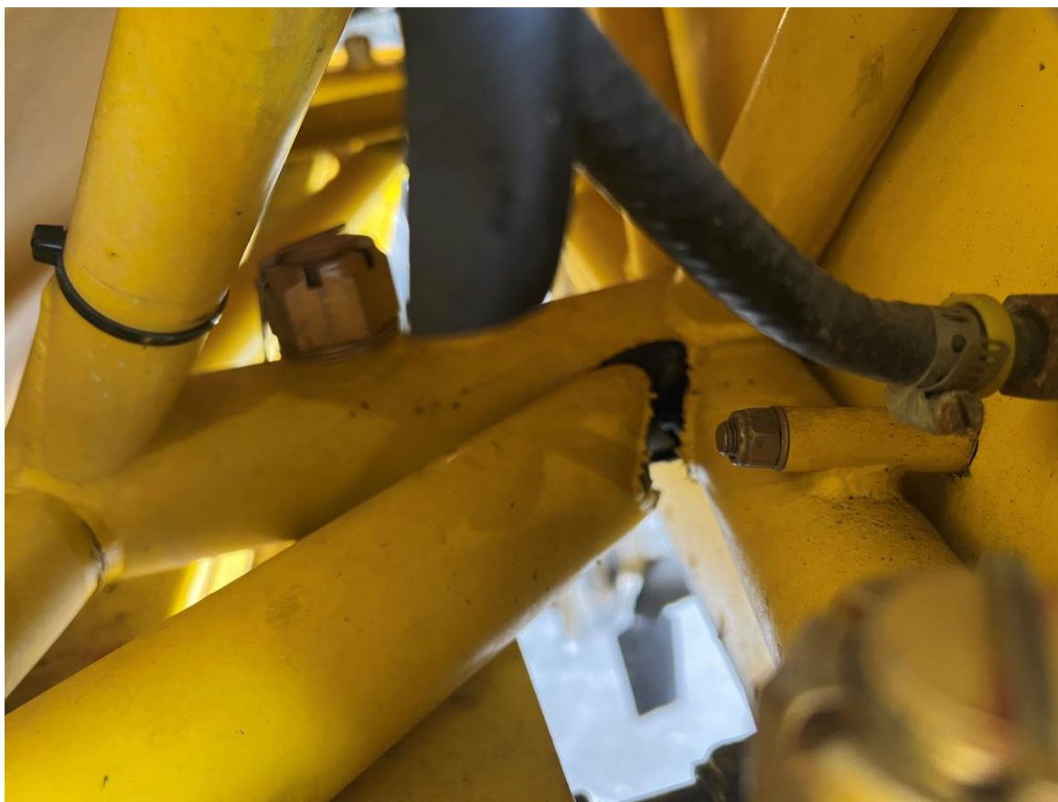
Photograph 1 - Left Tubular Cluster (Courtesy of TriState Aviation)
