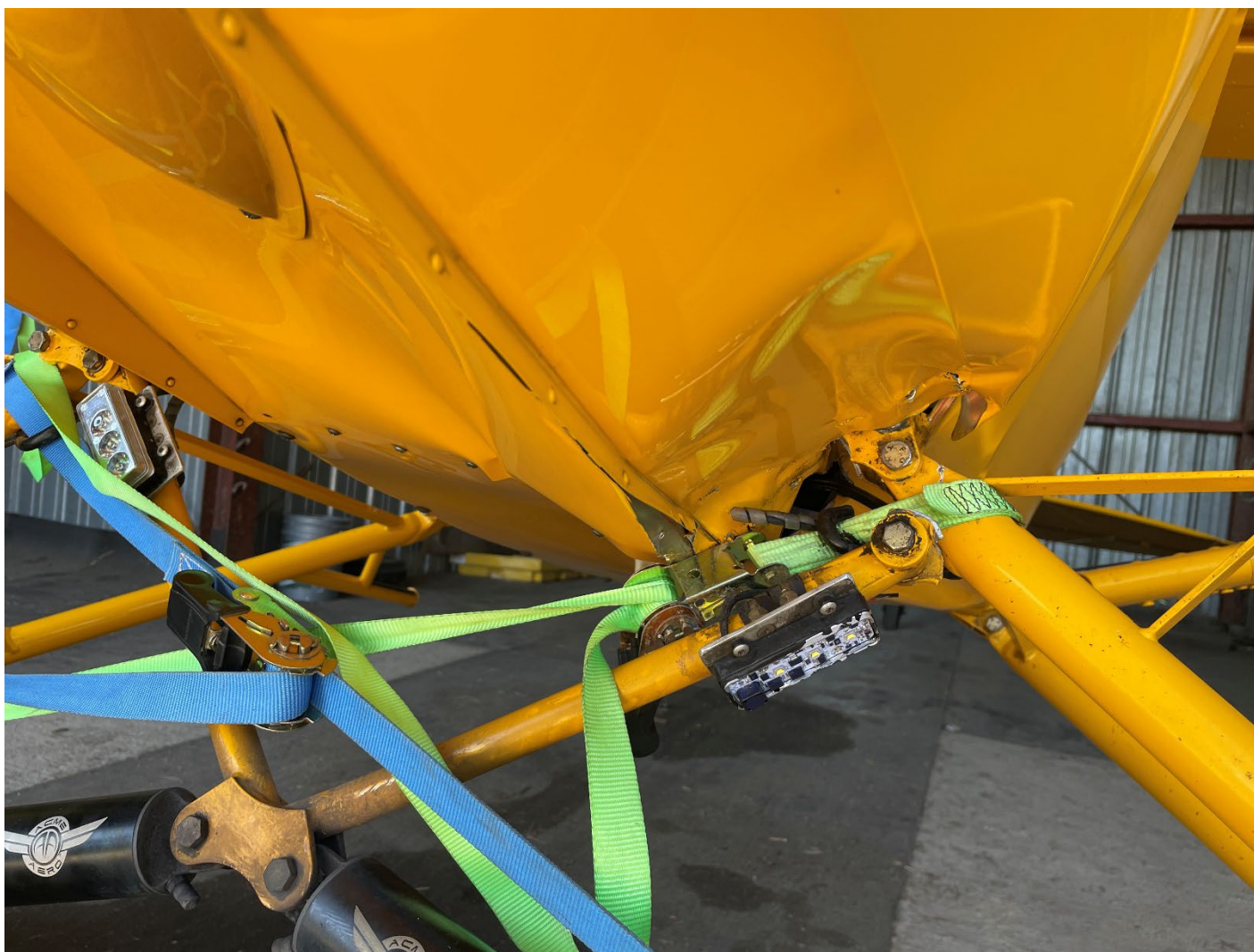
Photograph 1 - Forward lower fuselage and right main landing gear attach area; localized skin crushing and wrinkling near the fractured gear fitting. (Courtesy of FAA)
