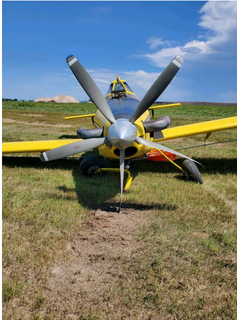
Photograph 3 - View looking aft of airplane at the accident site (Courtesy of FAA)
