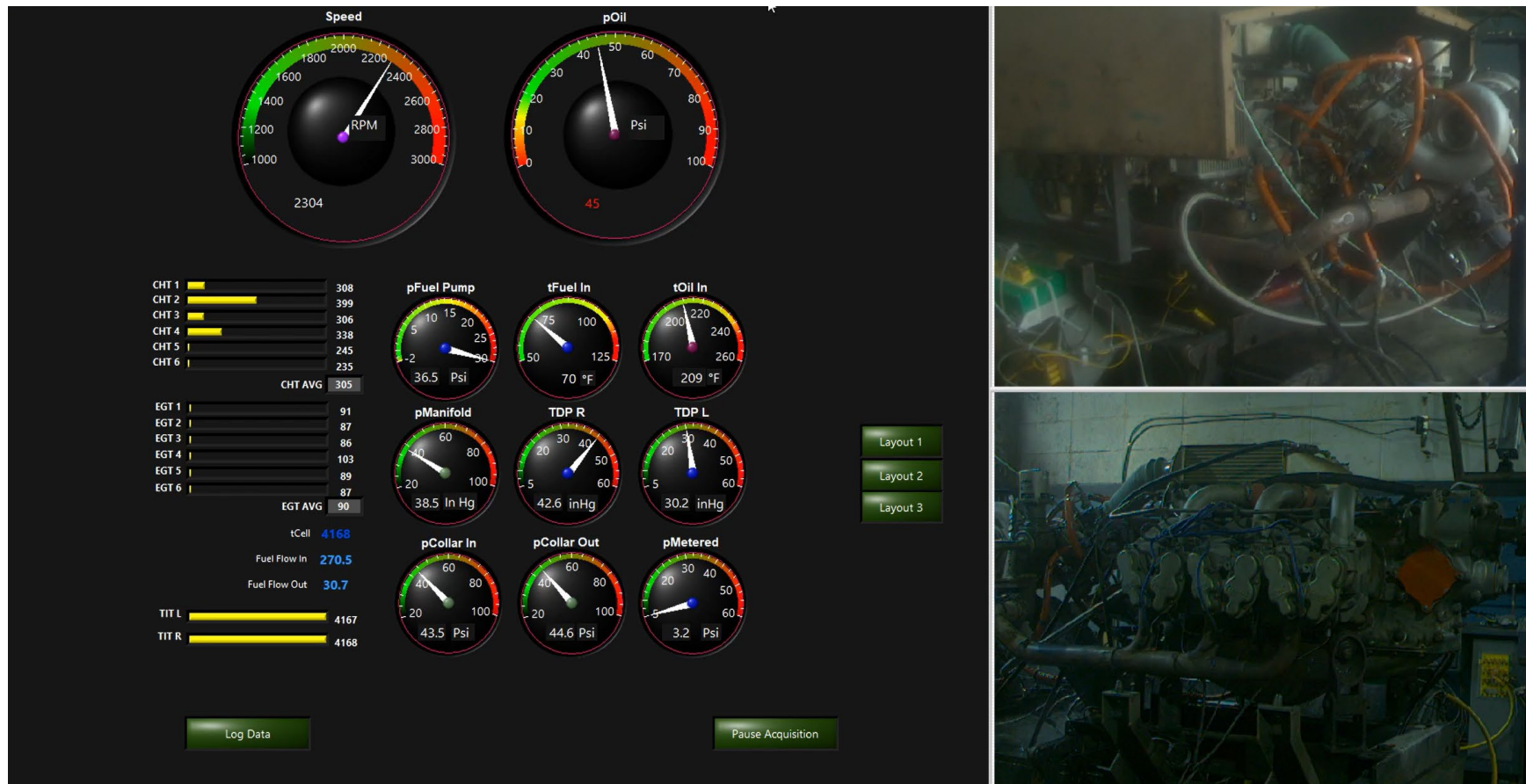
Photograph 6 - Right engine test run image (NTSB Photo)
