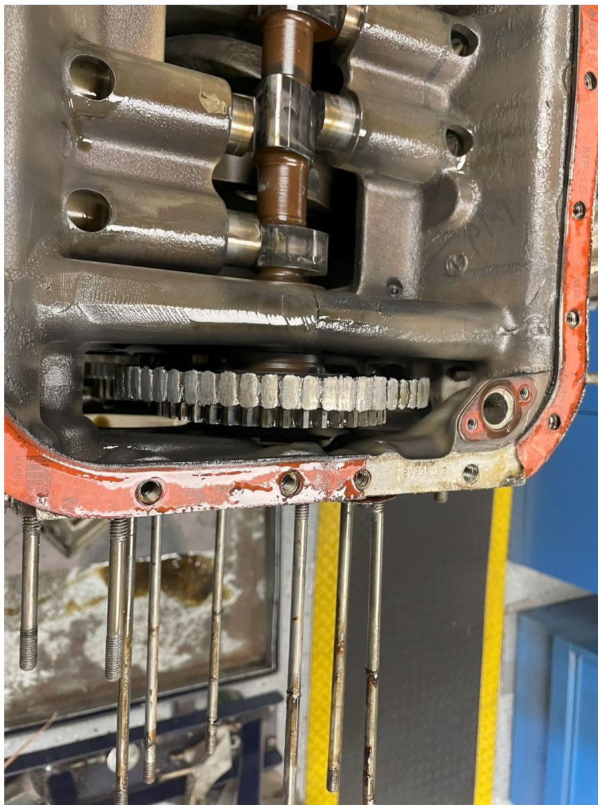
Photograph 8 - Left engine camshaft gear (NTSB Photo)
