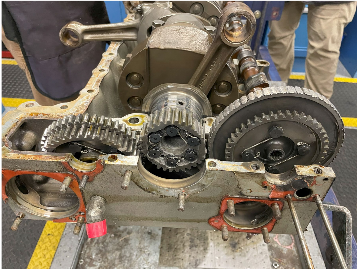
Photograph 9 - Left engine accessory gears (NTSB Photo)
