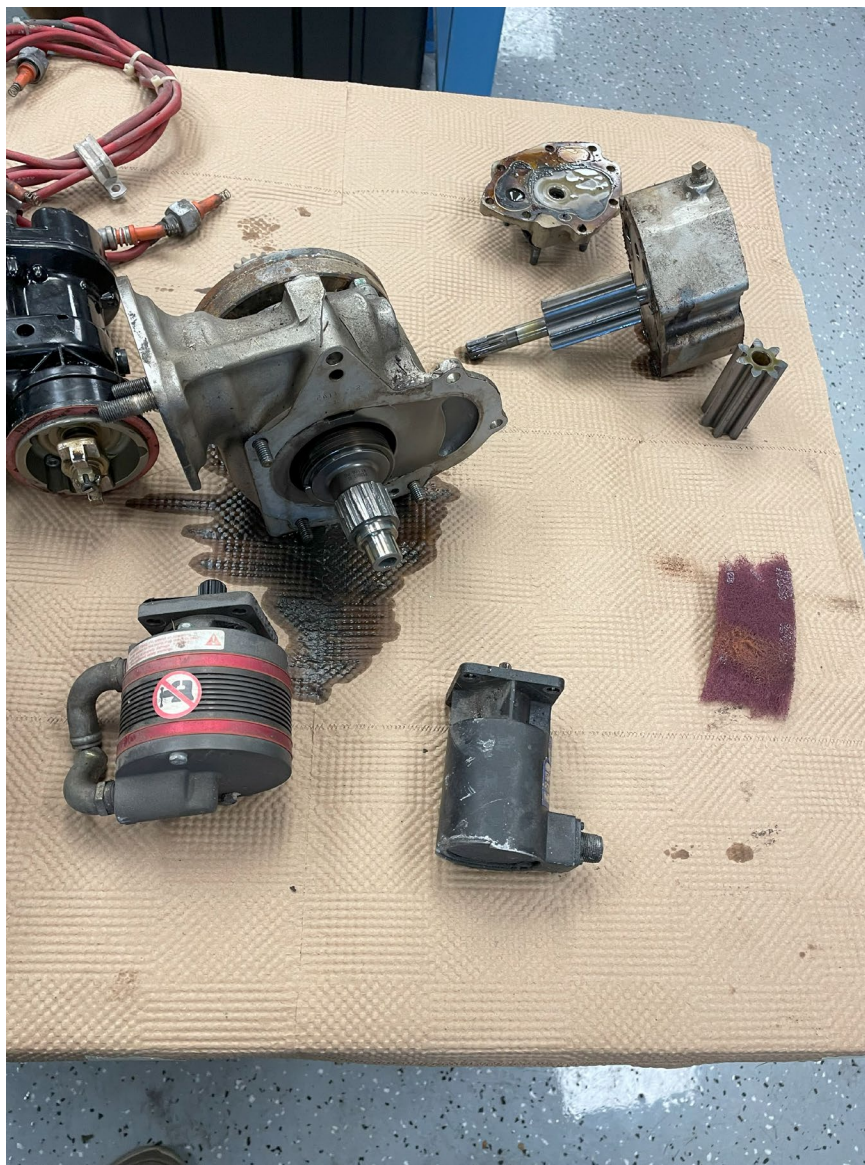
Photograph 10 - Left engine starter drive adapter (NTSB Photo)
