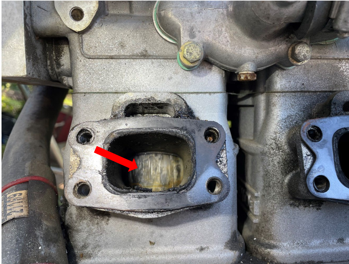
Photograph 3 - Scoring on Piston (Taken by NTSB)
