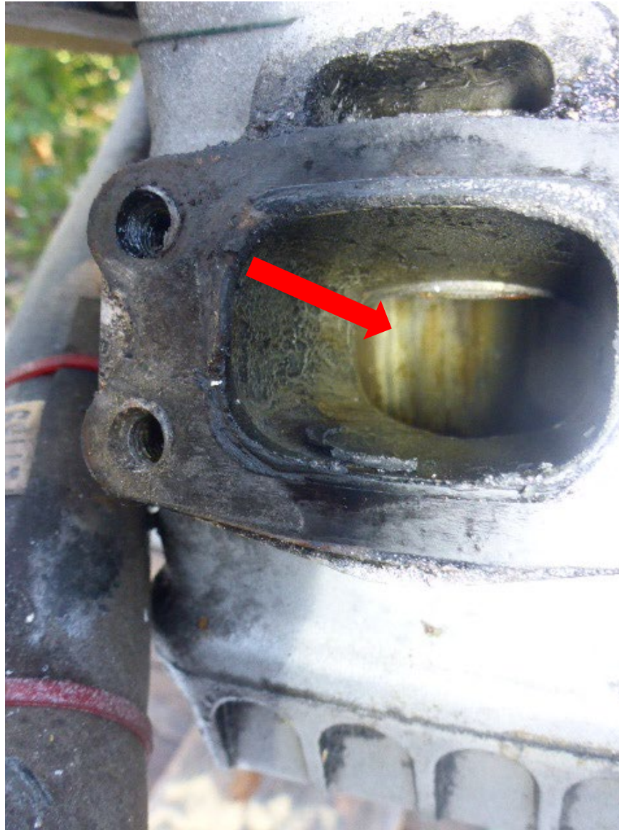
Photograph 4 - Scoring on Cylinder Wall (Taken by NTSB)
