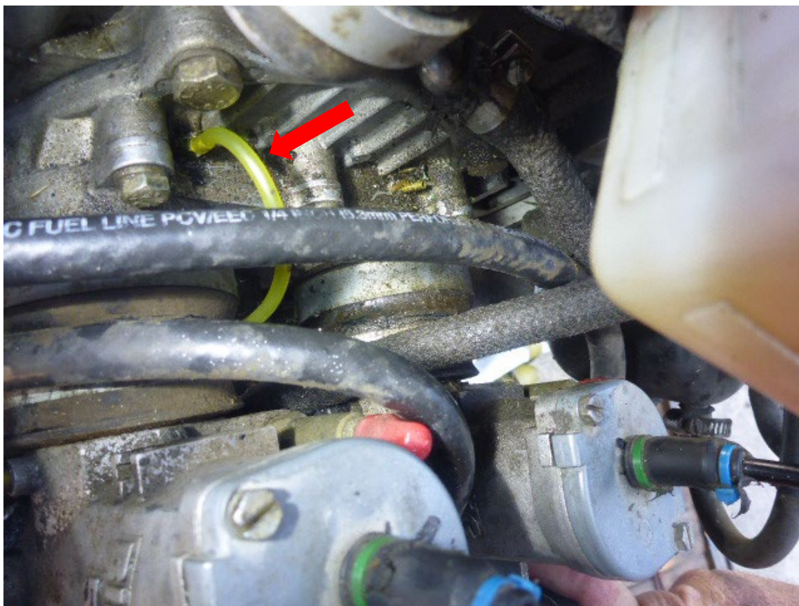
Photograph 5 - Newly Installed Oil Injection Line by Owner (Taken by NTSB)
