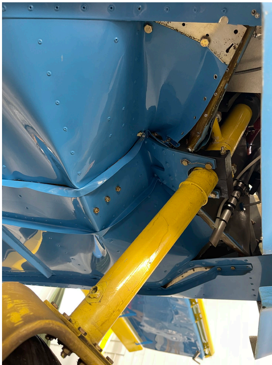
Photo 2 – Close up view of damaged fuselage and firewall (Courtesy of aircraft owner)
