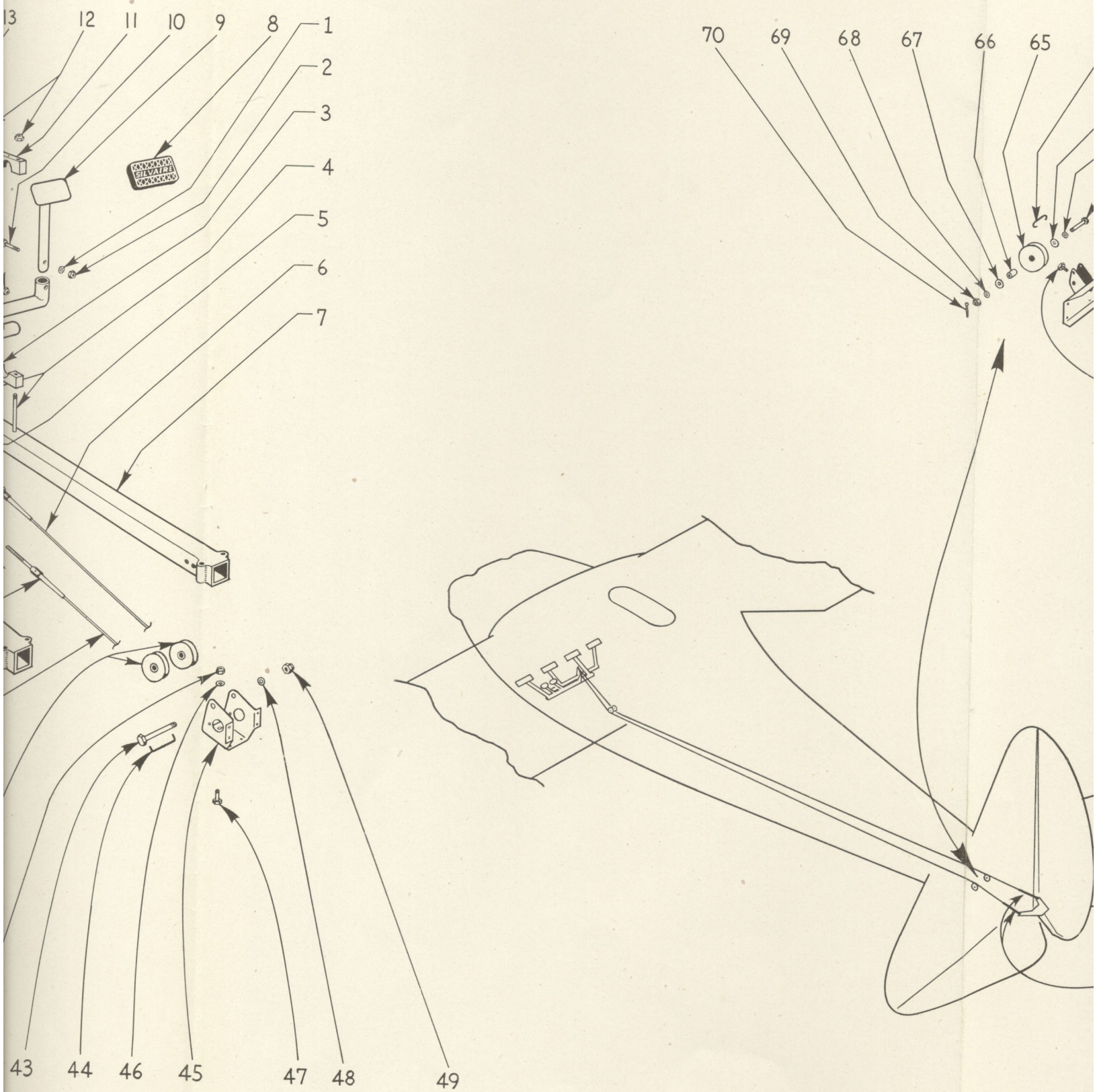
FIGURE No.14 RUDDER CONTROL
