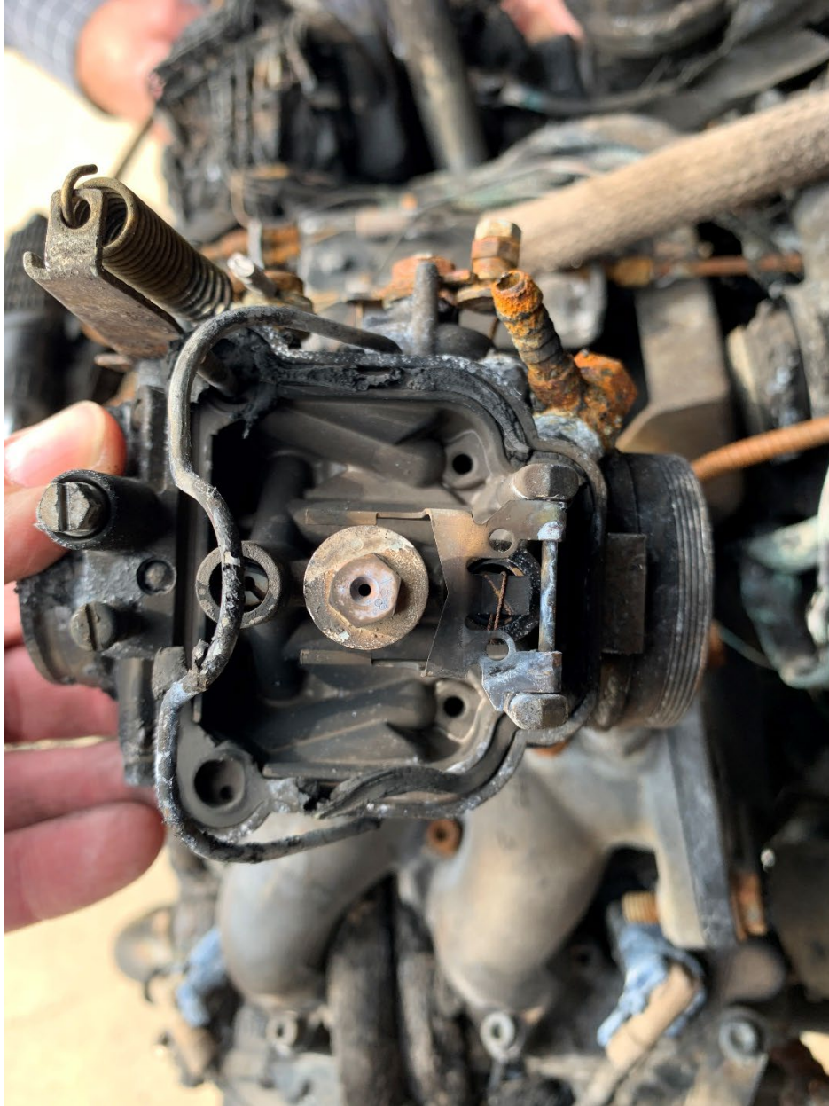
Photo 9: Bottom View of Left Carburetor (Source – NTSB IIC)
