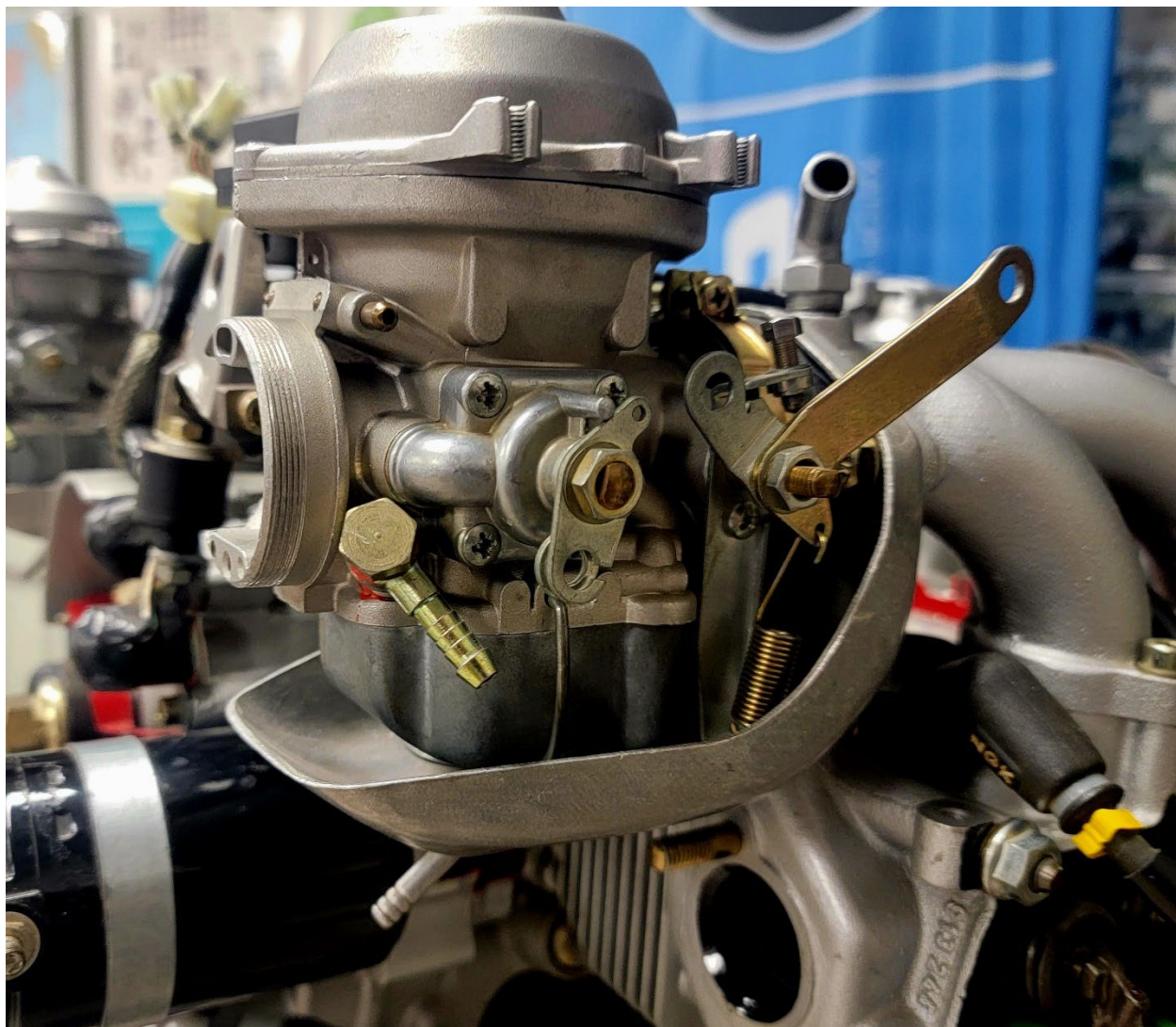
Photo 2: Exemplar Carburetor Drip Tray Installation (Source – Rotech Flight Safety Inc.)
