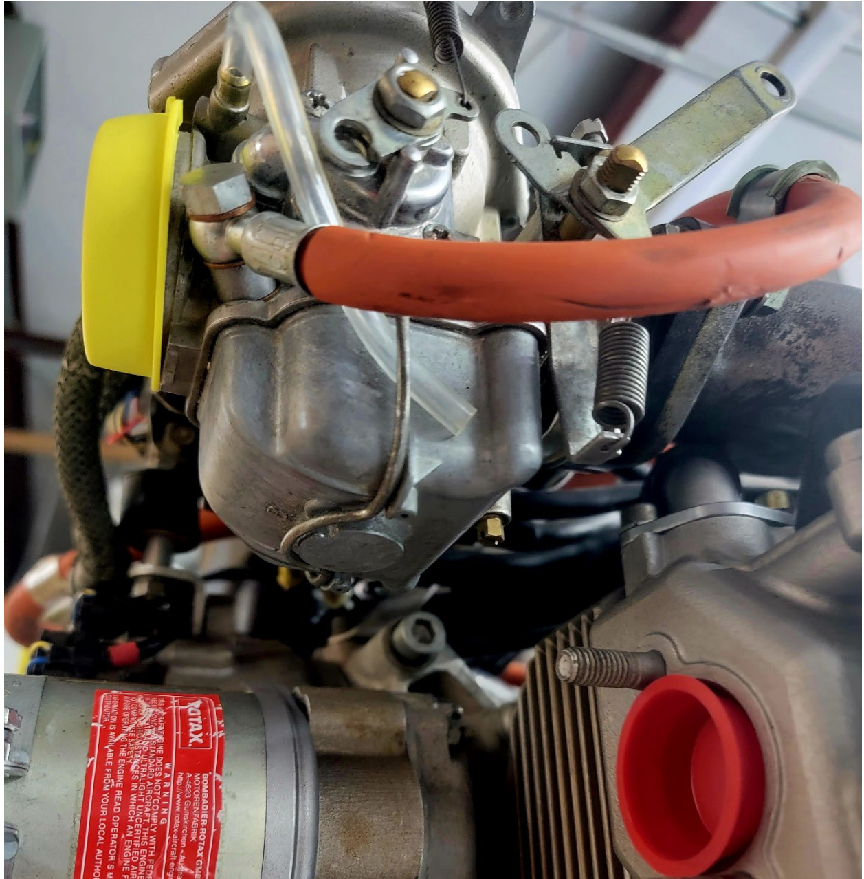
Photo 1: Exemplar Carburetor with Secured Carburetor Bowl Retention Clip Position (Source – Rotech Flight Safety Inc.)
