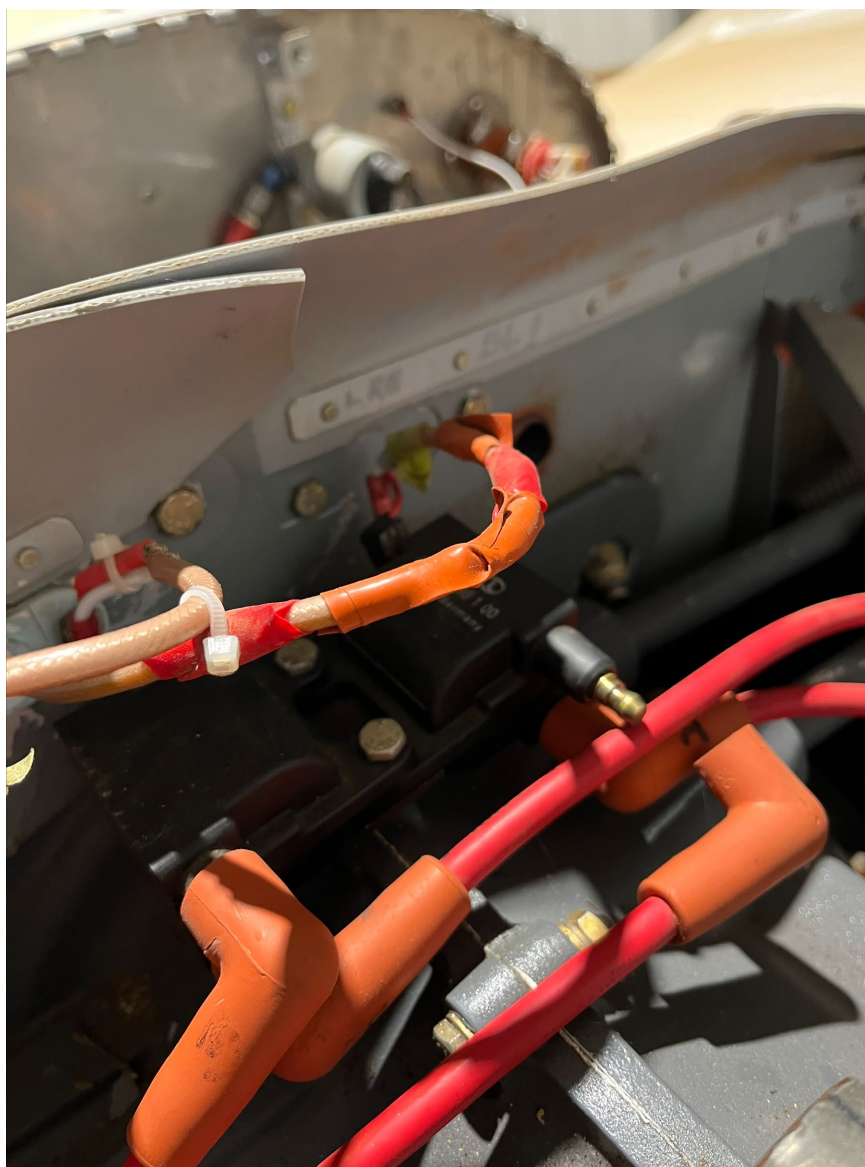
Photograph 3 - Ignition Lead (Courtesy of FAA)
